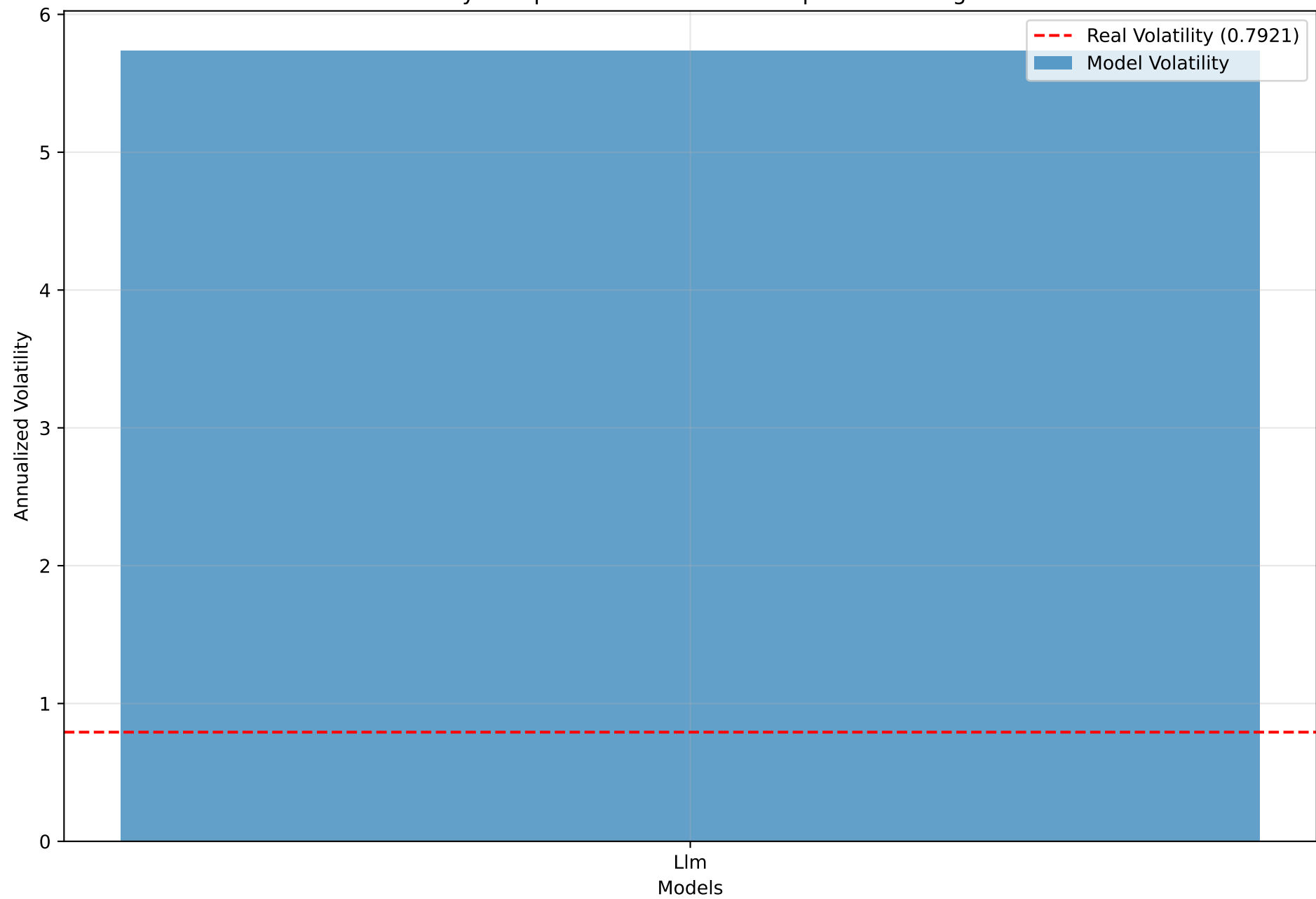
Volatility Comparison - Llm Knob Comp0 Shift 1.0Sigma
