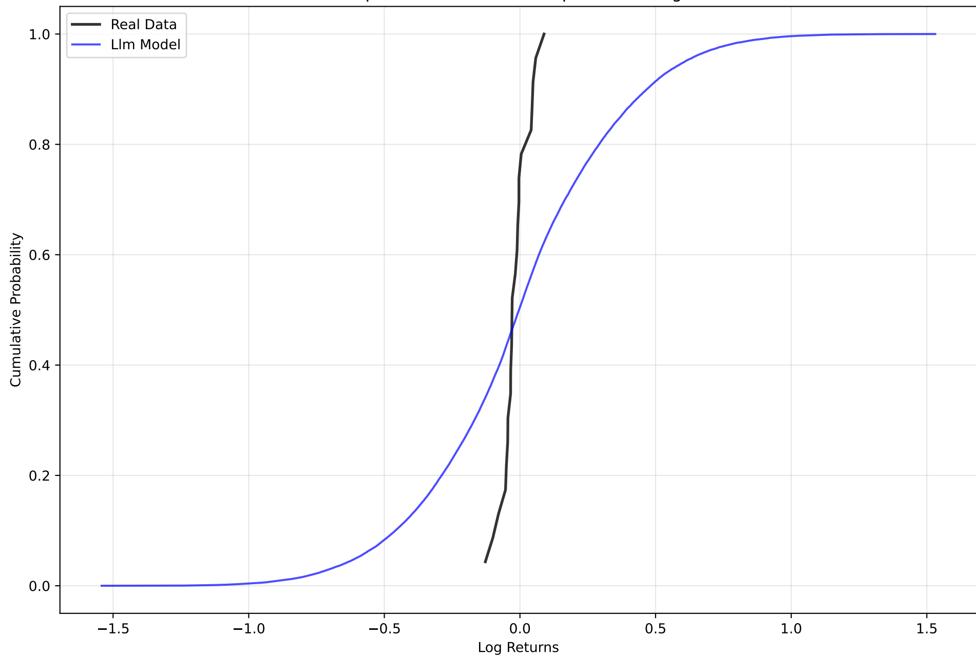
ECDF Comparison - Llm Knob Comp0 Shift 2.0Sigma Mode
