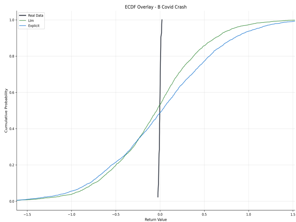
ECDF Overlay - covid_crash
