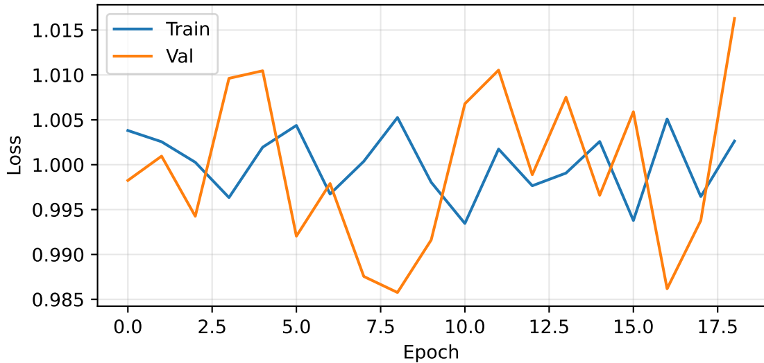
Losses: ddpm_evaluation_20250812_233700
