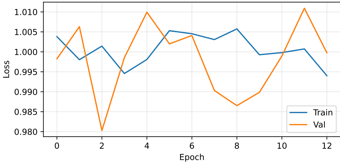
Losses: ddpm_evaluation_20250813_112116
