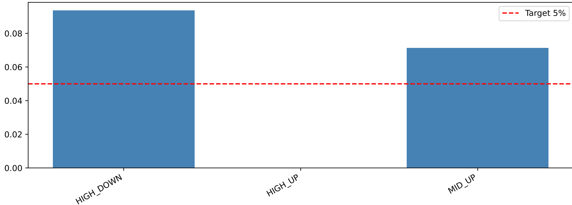
COVID: Conditional VaR95 coverage — explicit_conditioned
