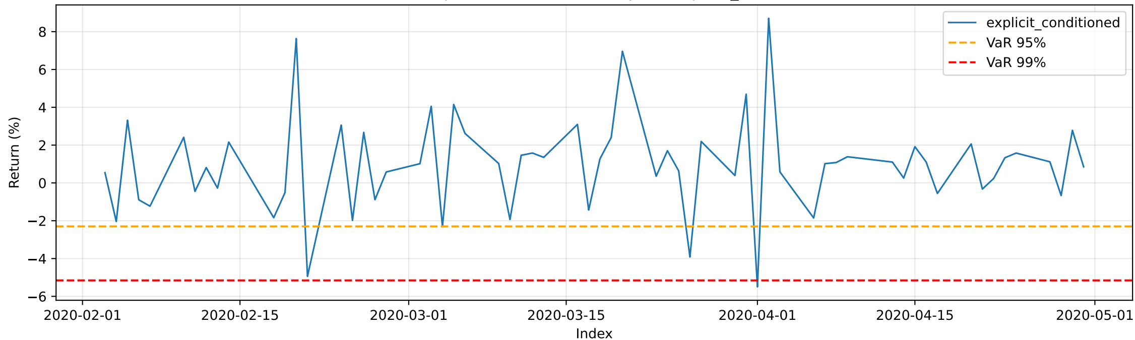
COVID: Sequence with VaR overlays — explicit_conditioned
