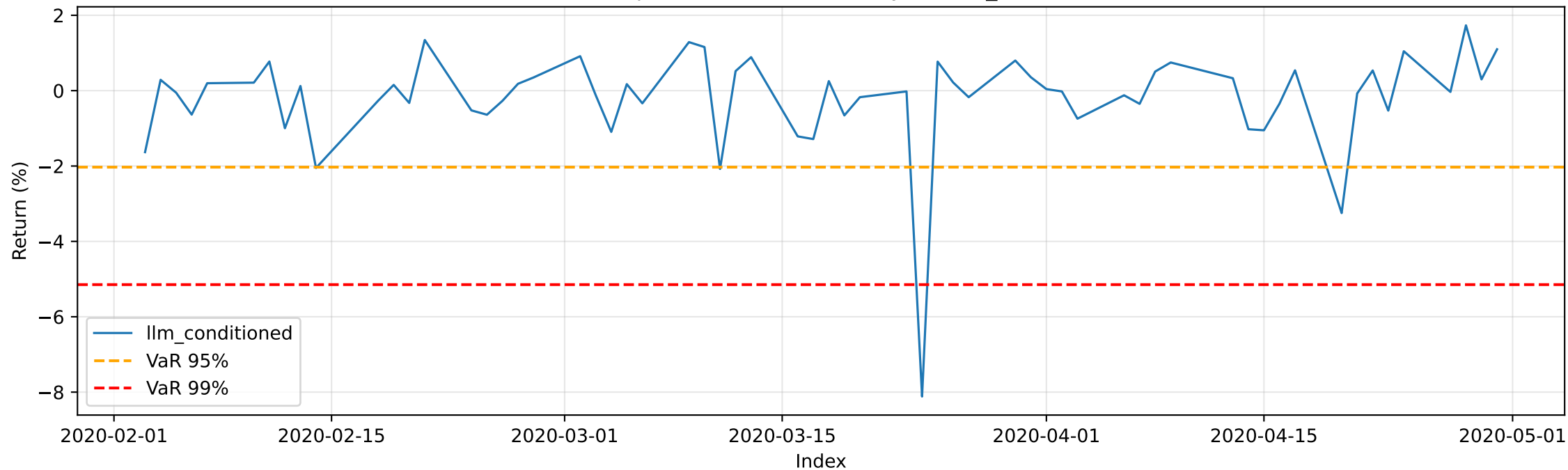
COVID: Sequence with VaR overlays — llm_conditioned
