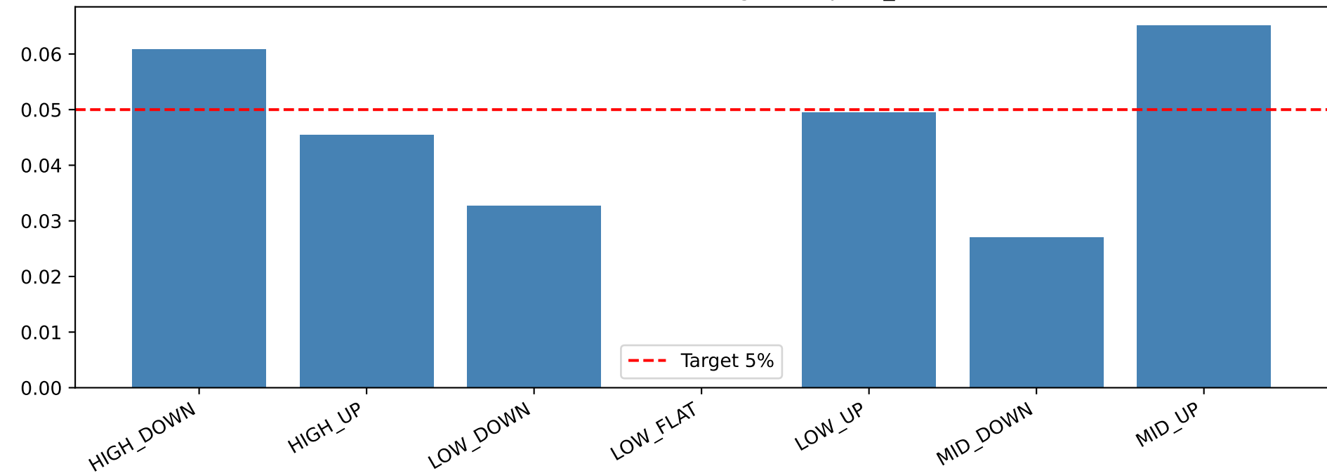
Calm: Conditional VaR95 coverage — explicit_conditioned
