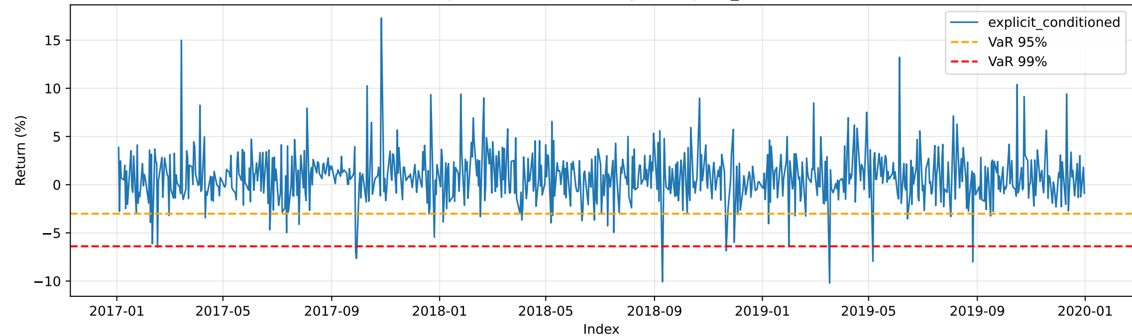
Calm: Sequence with VaR overlays — explicit_conditioned
