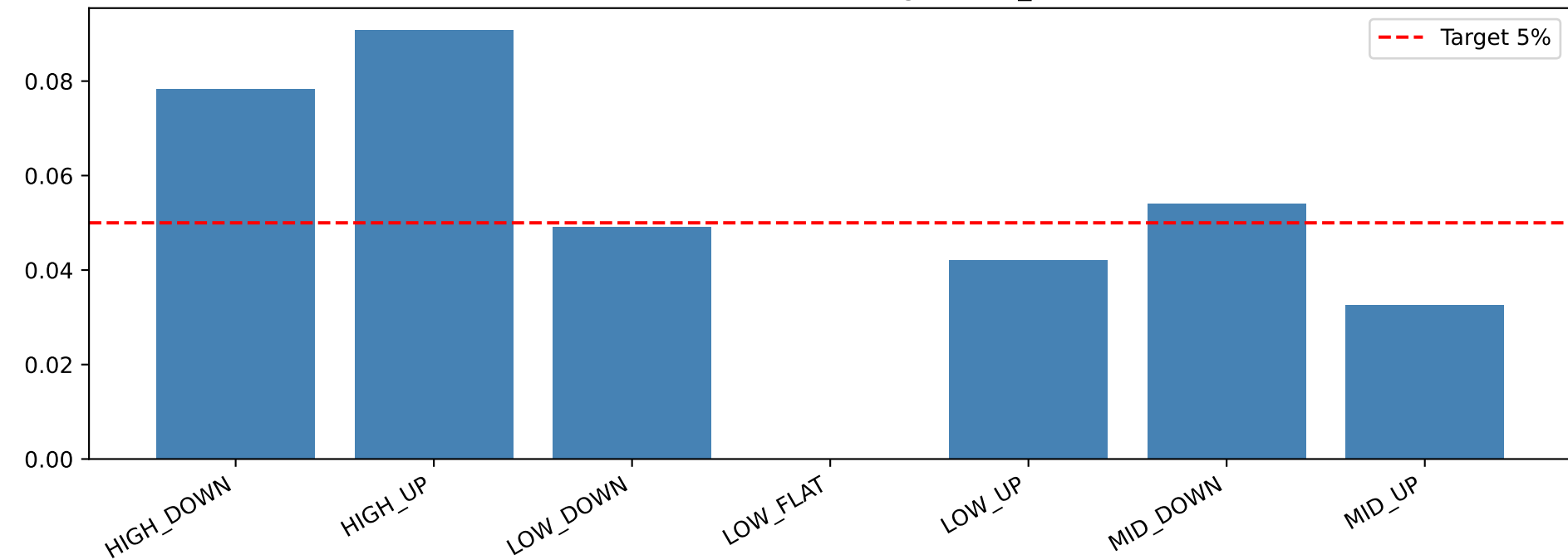
Calm: Conditional VaR95 coverage — llm_conditioned
