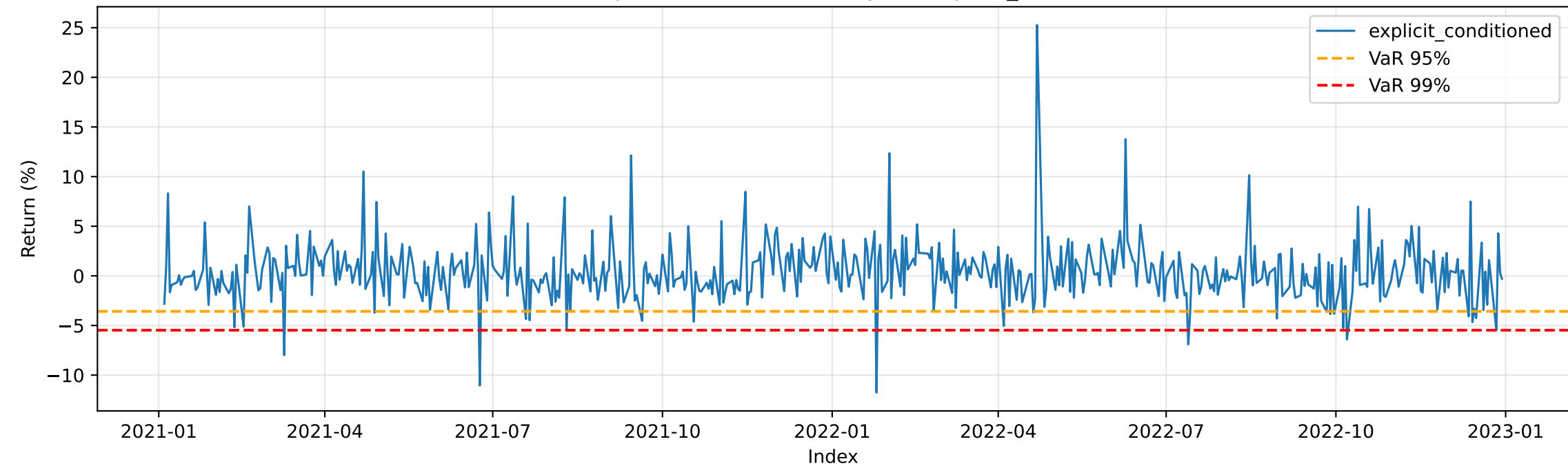
Post: Sequence with VaR overlays — explicit_conditioned
