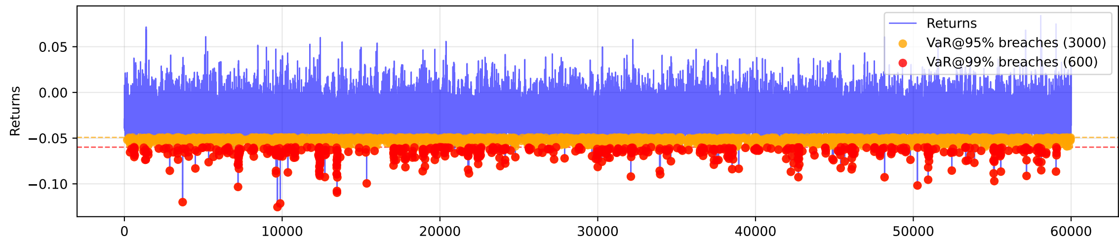
explicit VaR Exceedances
