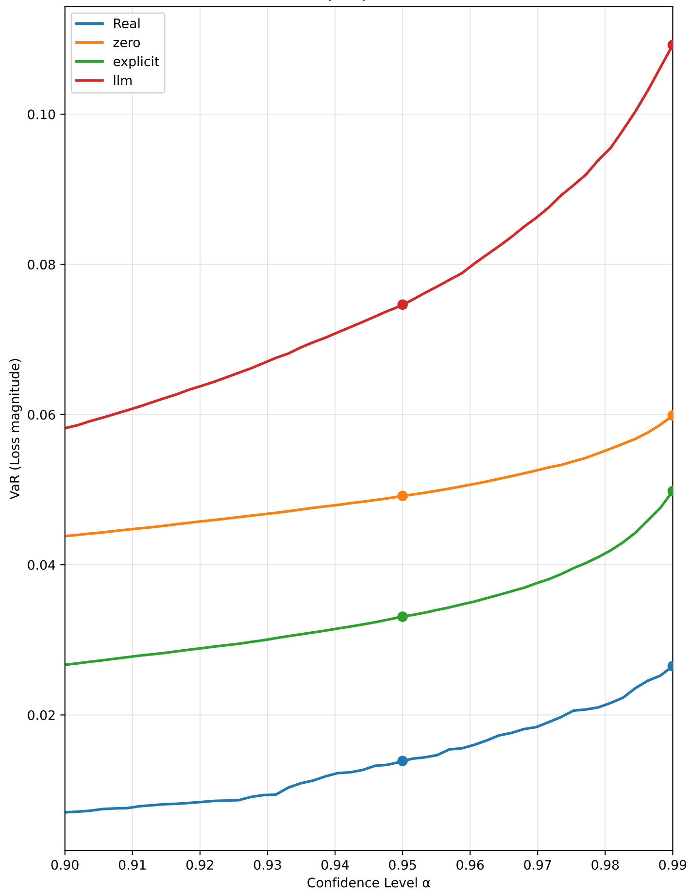
Value at Risk (VaR) Curves - PreCOVID
