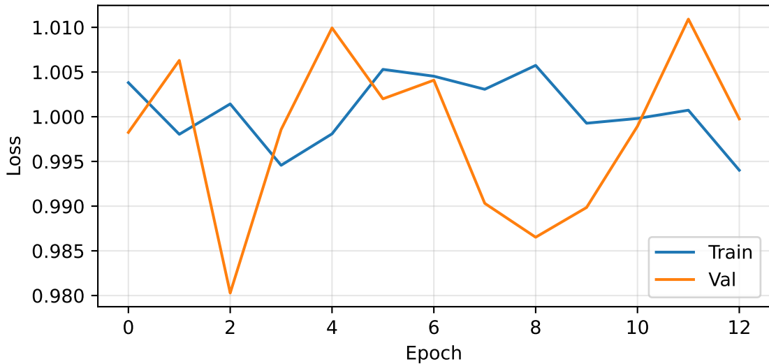
Losses: ddpm_evaluation_20250813_112116
