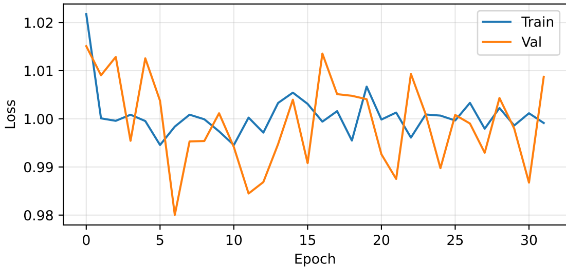
Losses: ddpm_evaluation_20250813_114508
