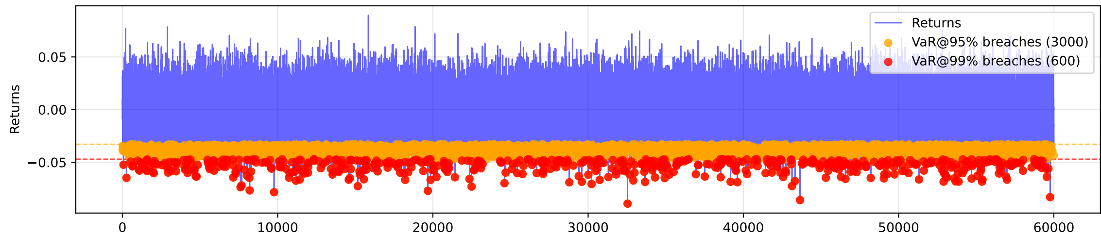
explicit VaR Exceedances
