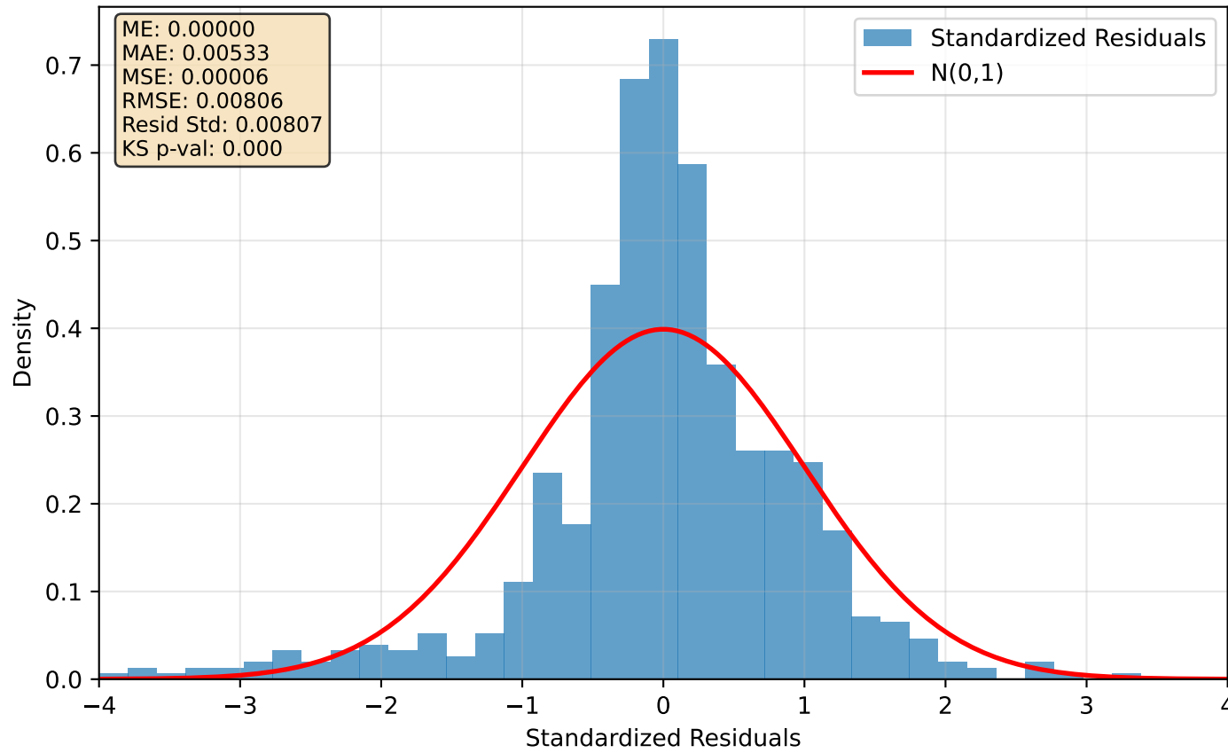
explicit Standardized Residuals
