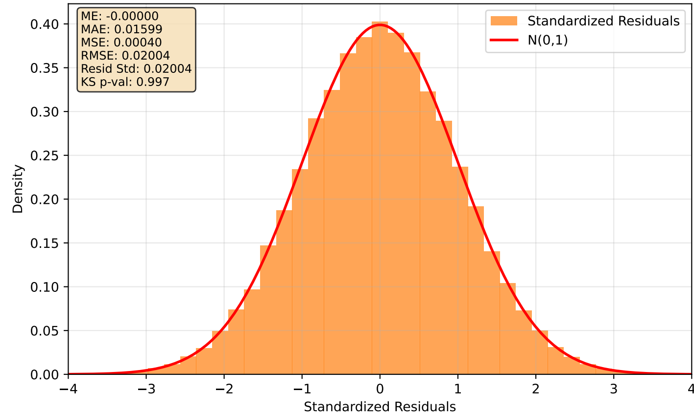
llm Standardized Residuals
