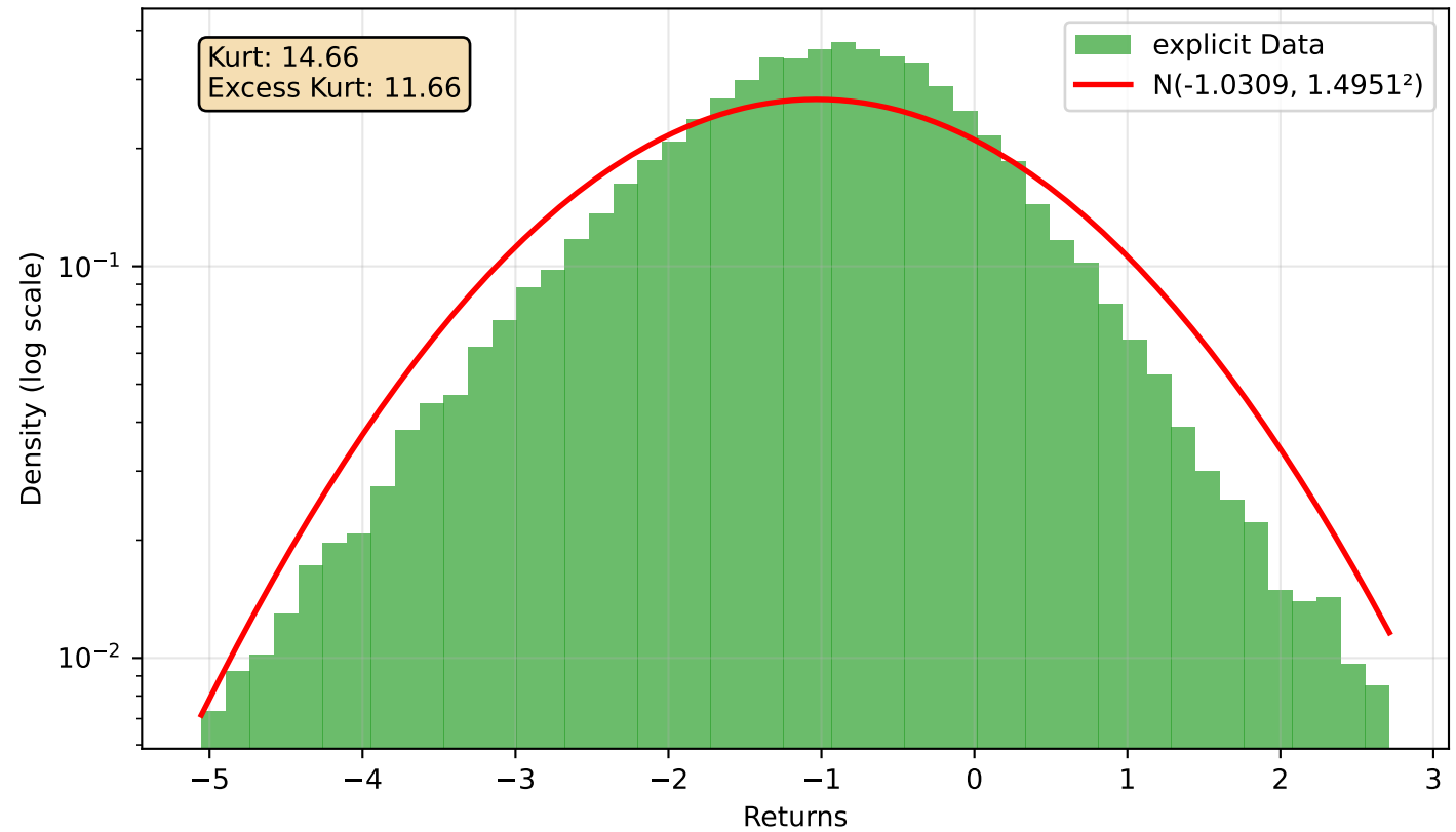
explicit Returns Distribution △ SUSPECT SCALE (std=1.495076, max|r|=24.176)
