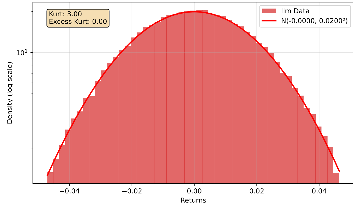
Ilm Returns Distribution
