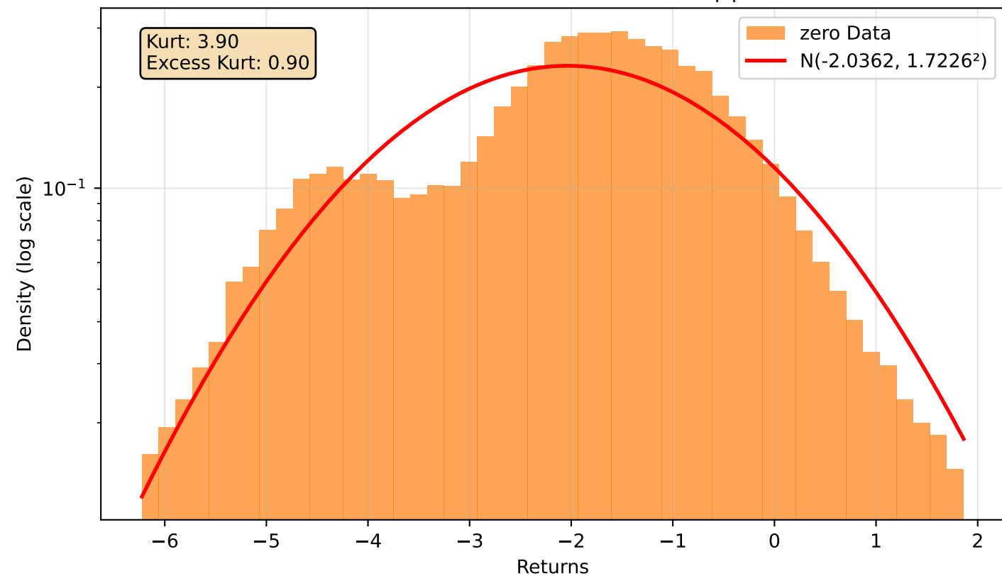
zero Returns Distribution △ SUSPECT SCALE (std=1.722581, max|r|=16.355)
