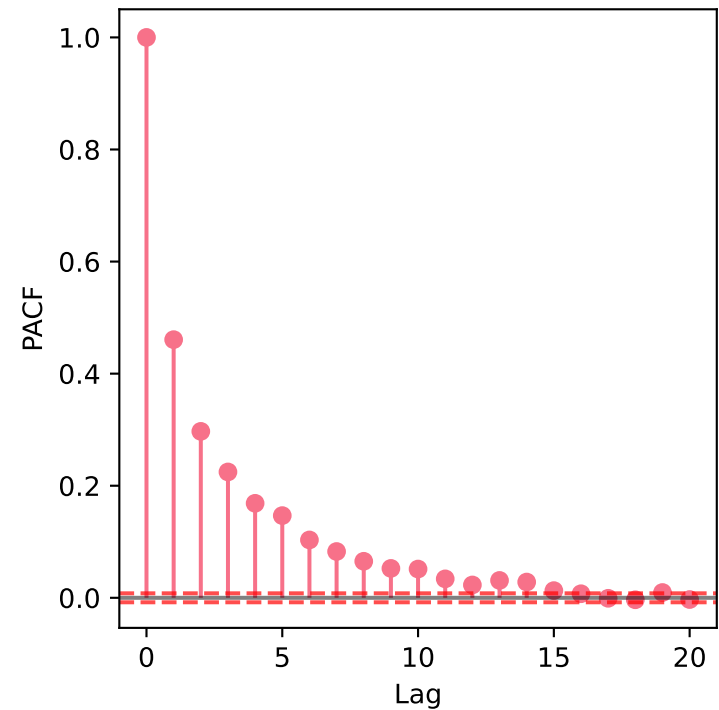
Ilm - PACF Squared Returns
