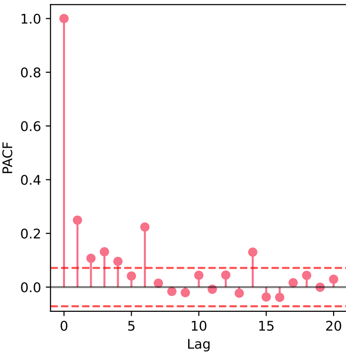
Real - PACF Squared Returns
