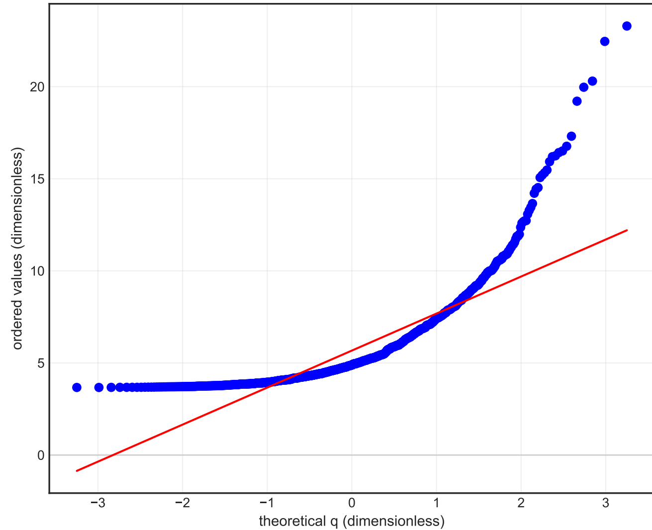
Q-Q right tail
