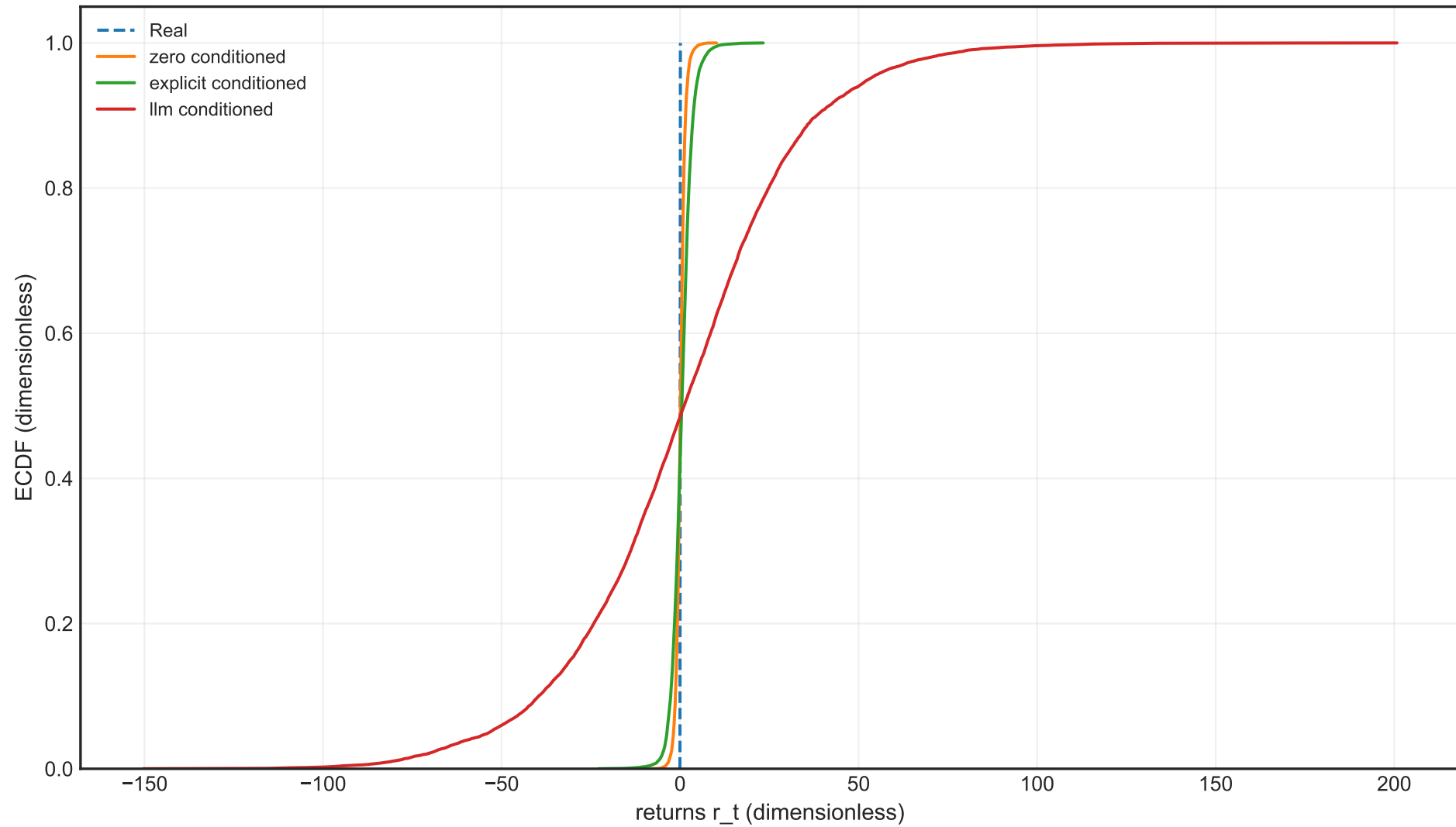
ECDF Overlay
