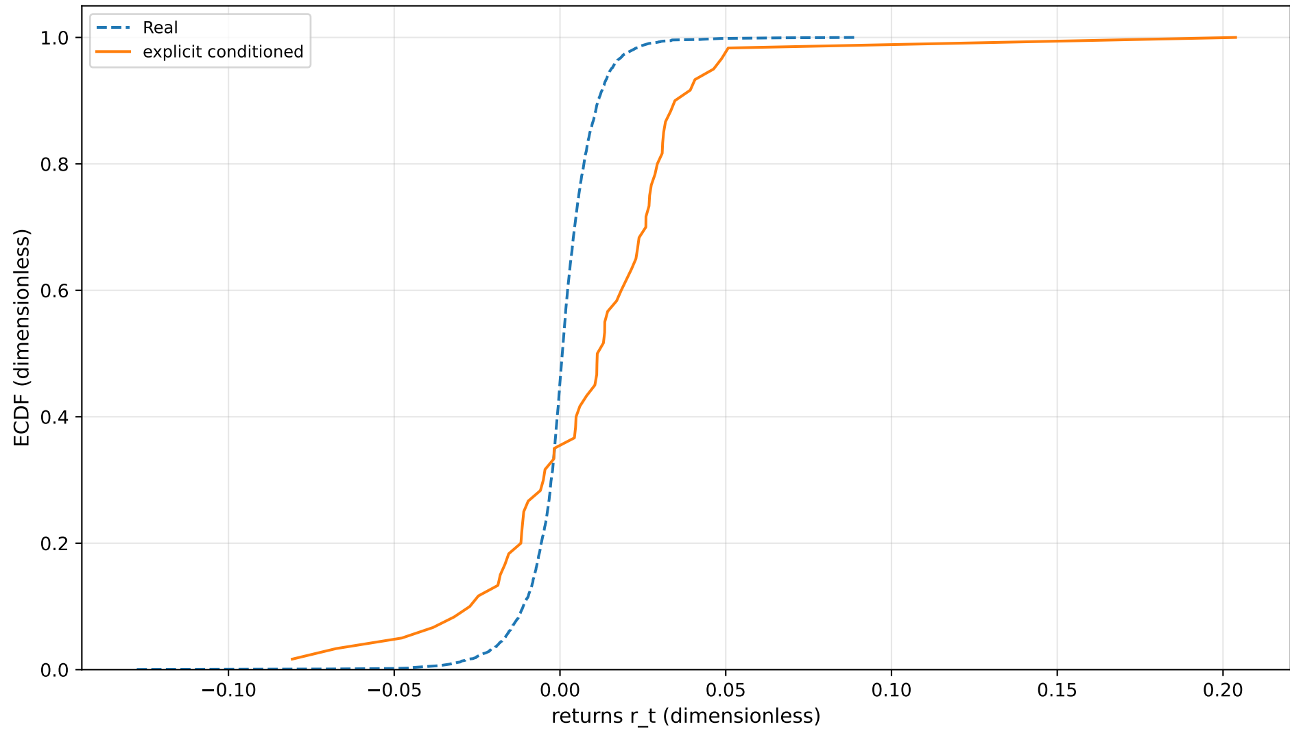
ECDF Overlay
