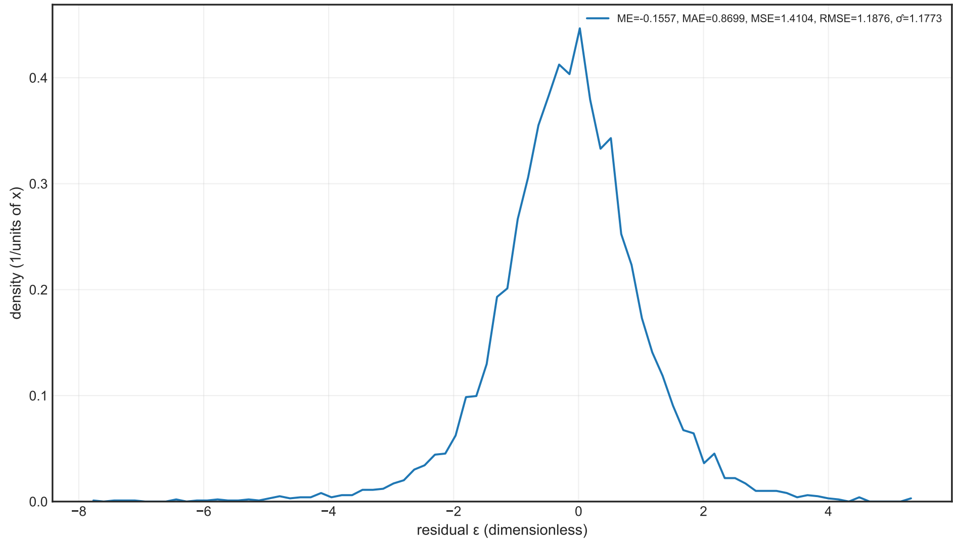
Residual Histogram — zero_conditioned
