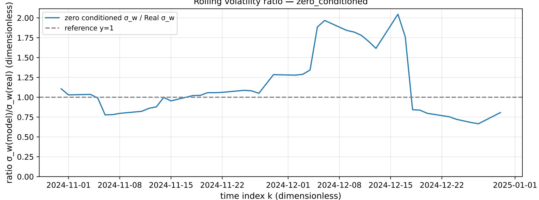
Rolling volatility ratio — zero_conditioned
