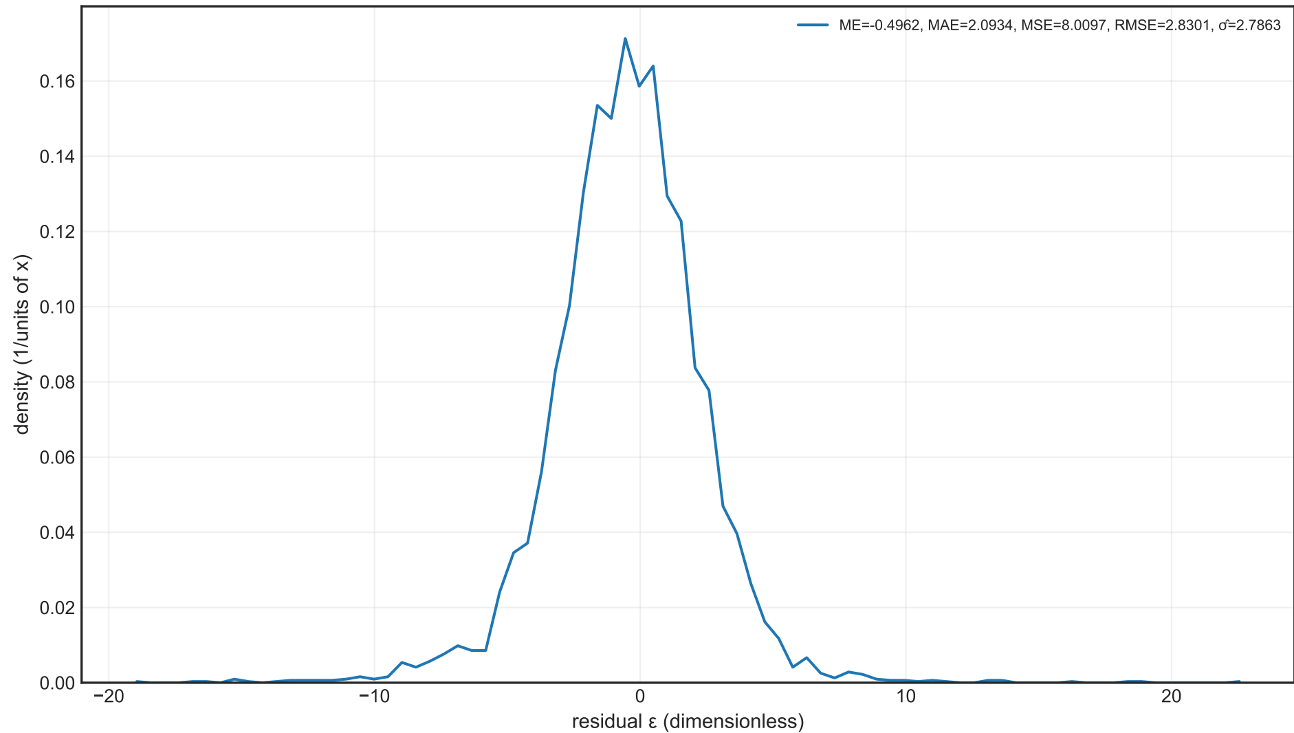
Residual Histogram — explicit_conditioned
