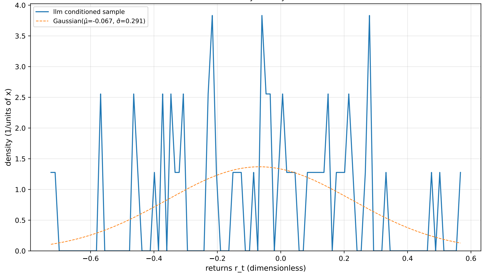
Density Overlay
