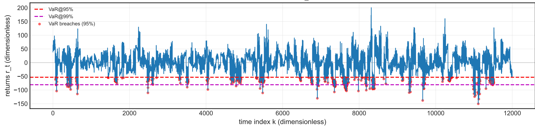
Exceedance timeline — llm_conditioned
