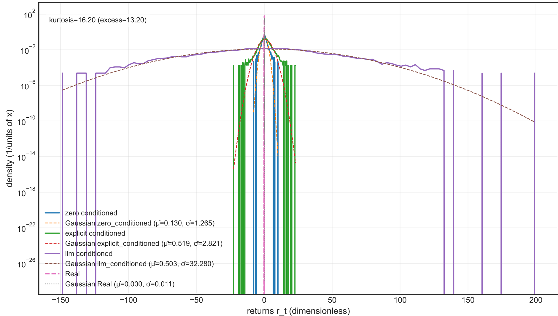
Histogram (log y-axis)
