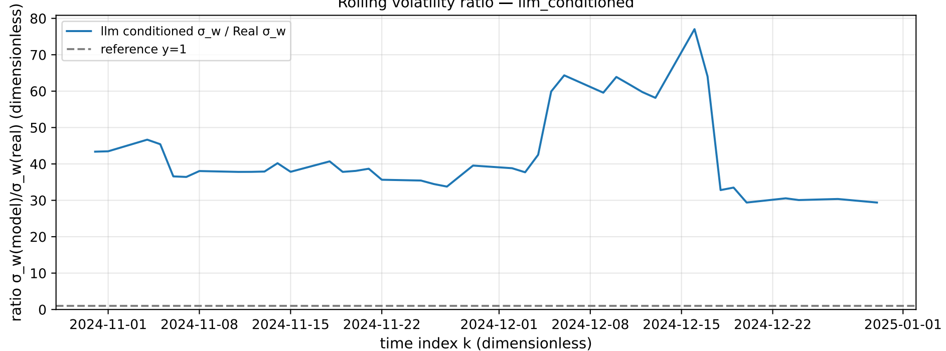
Rolling volatility ratio — llm_conditioned
