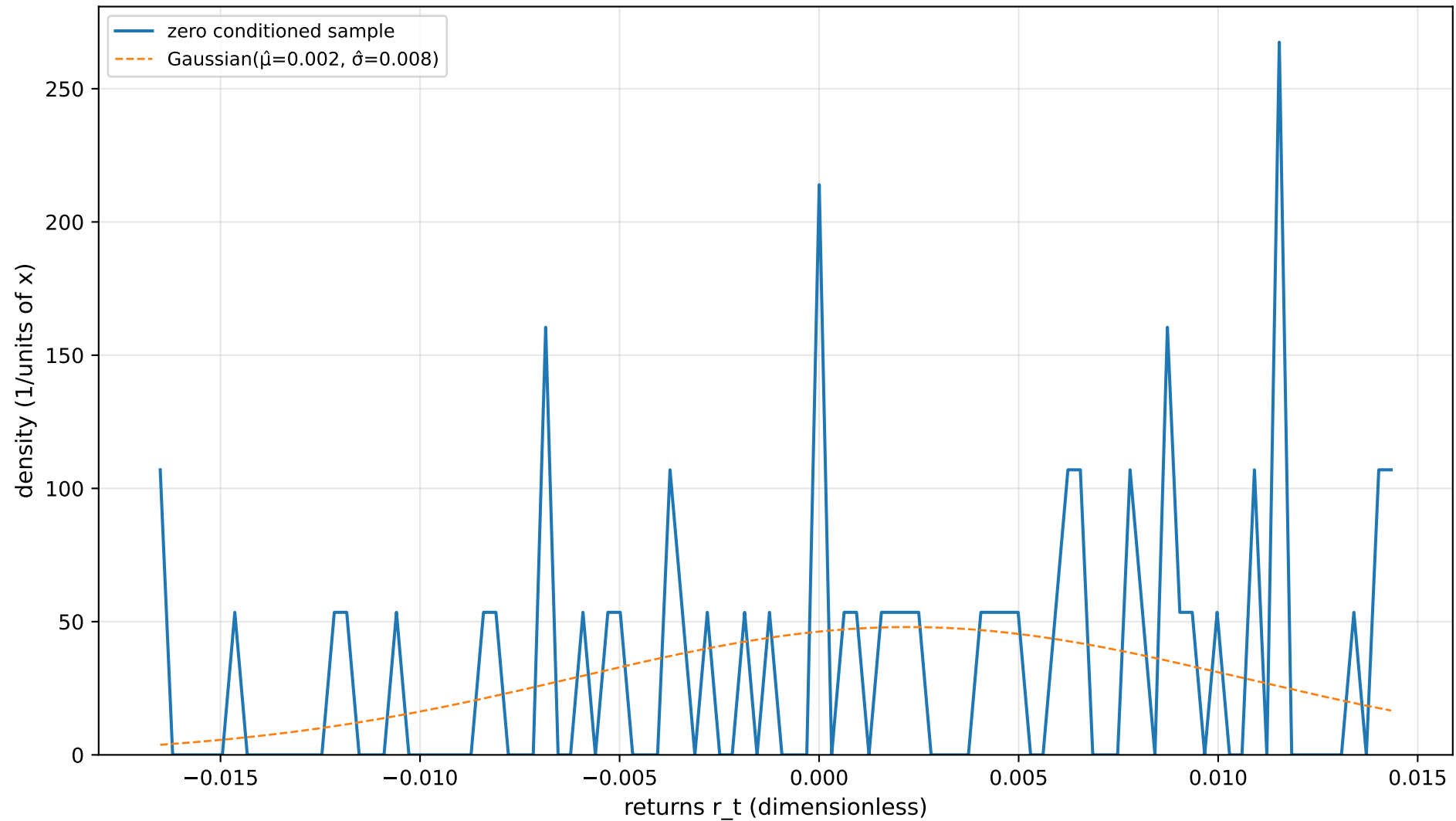
Density Overlay
