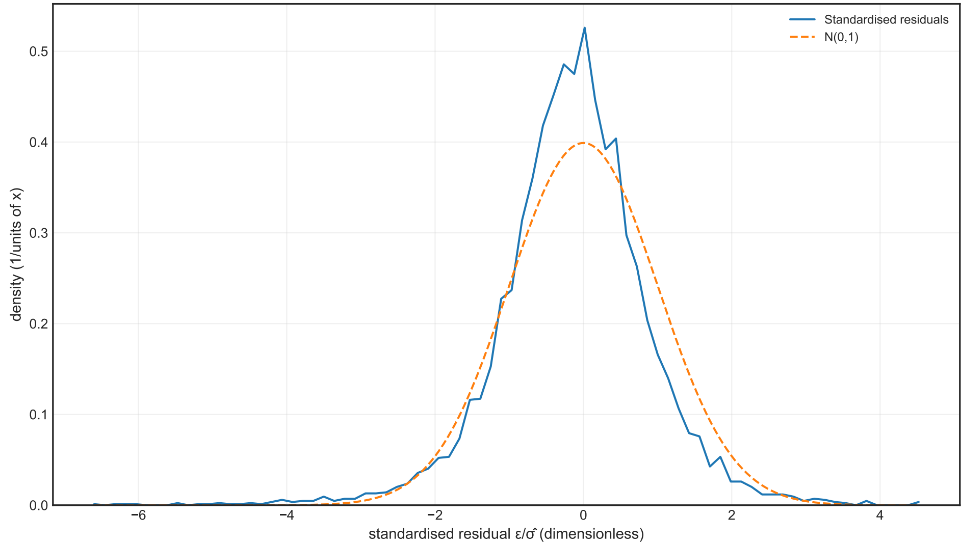
Standardised residuals vs N(0,1)
