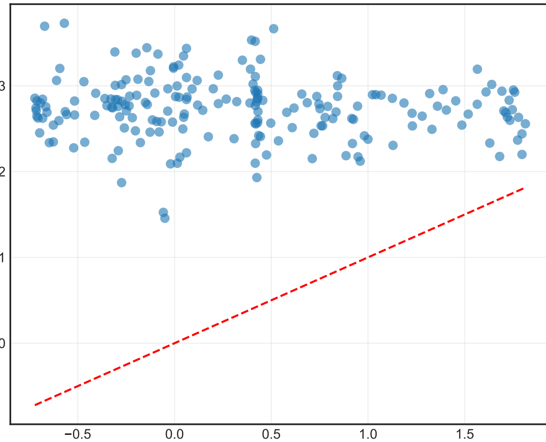
Target vs Realized
