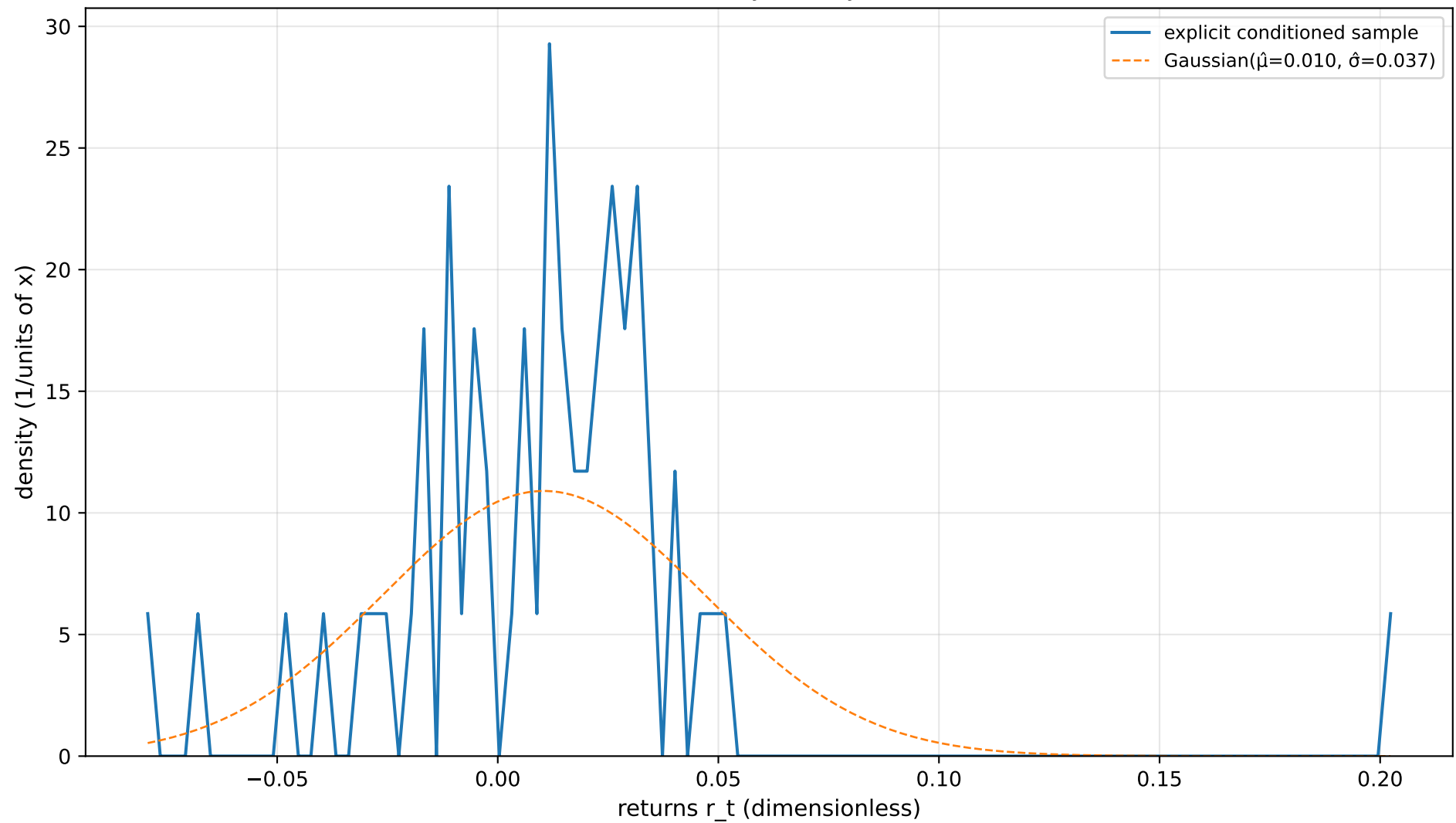
Density Overlay
