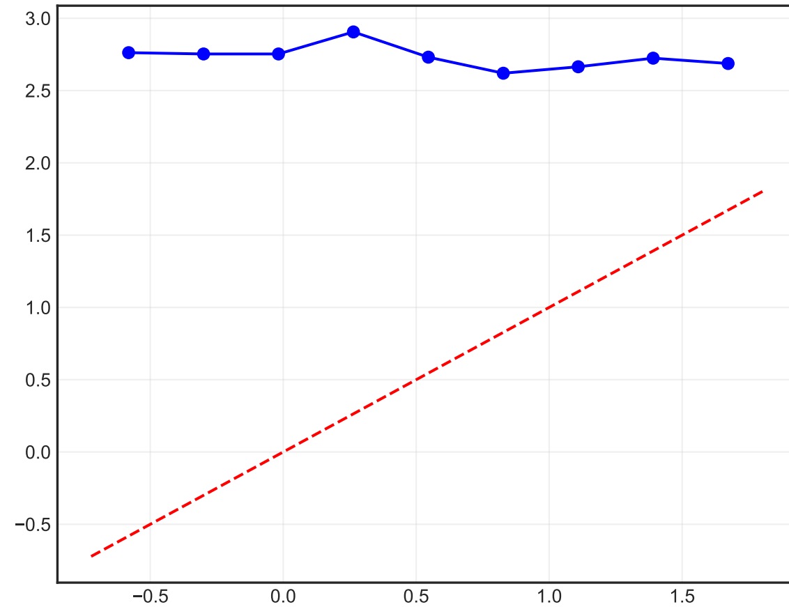
Reliability
