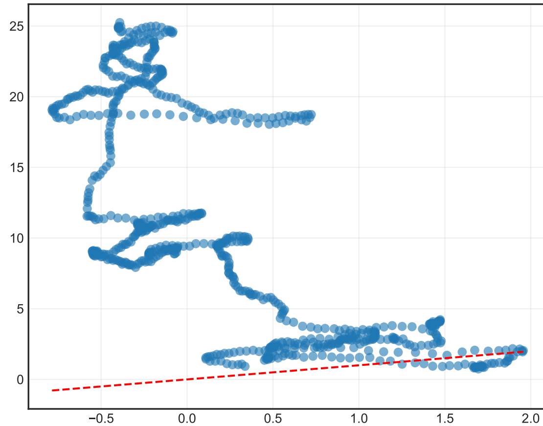
LLM Probe Scatter (MAE=10.711, R2=-389.289)
