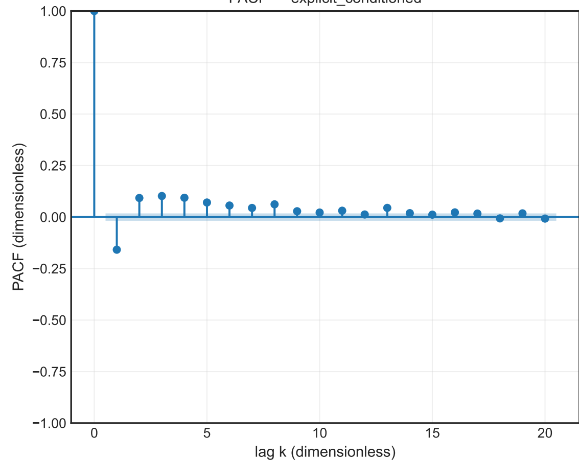
PACF (squared) — explicit_conditioned
