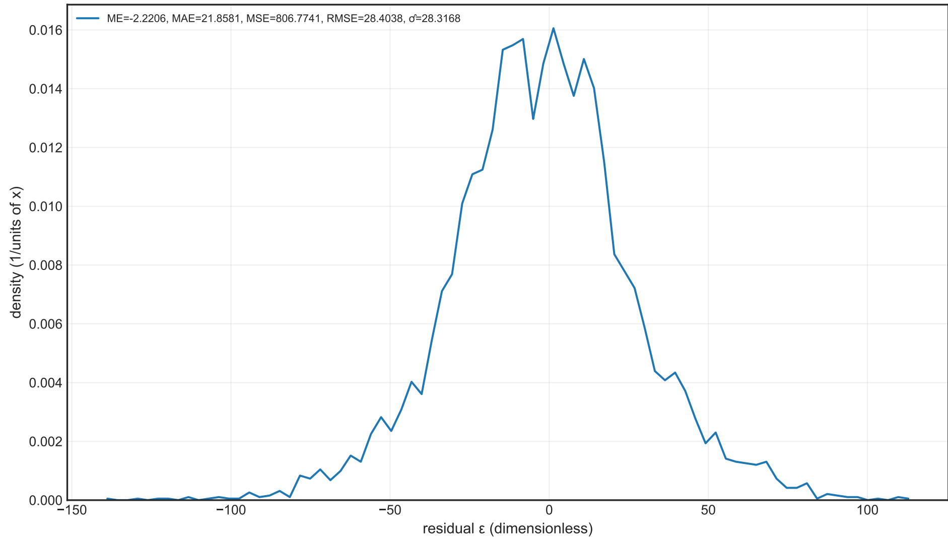
Residual Histogram — llm_conditioned
