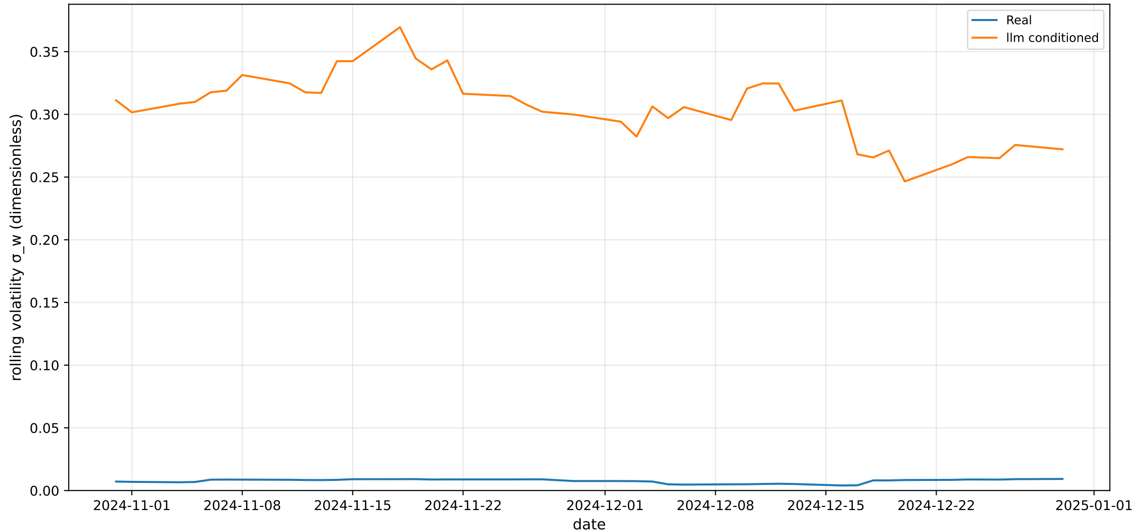
Rolling Volatility (window=20)
