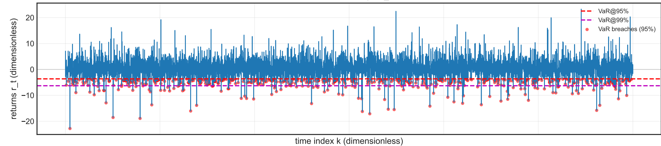
Exceedance timeline — llm_conditioned
