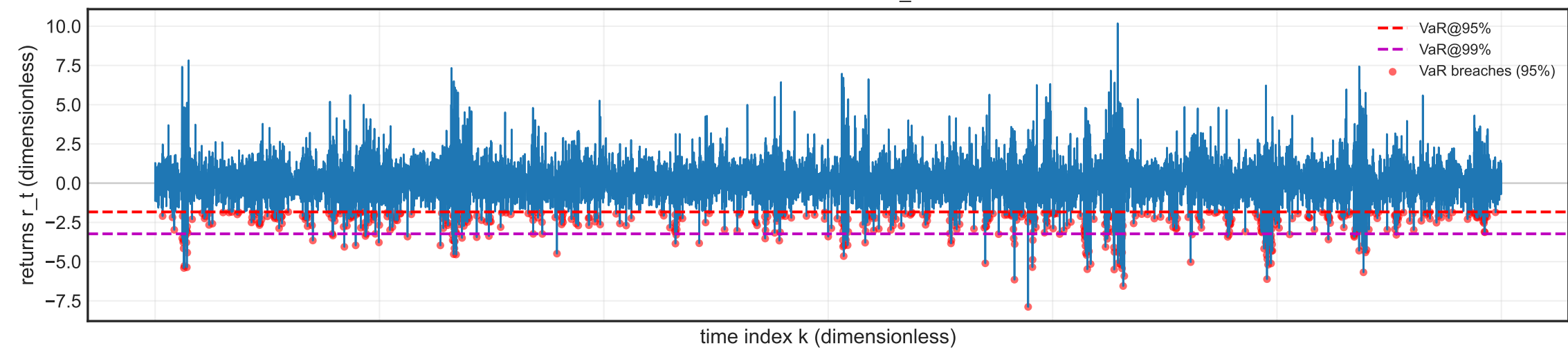
Exceedance timeline — explicit_conditioned
