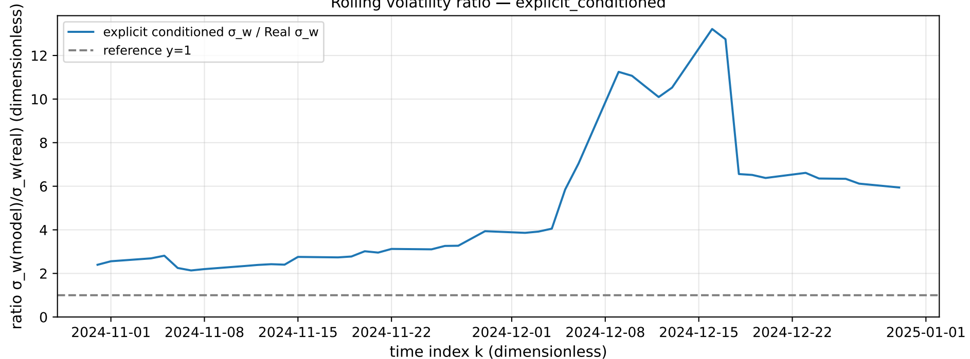
Rolling volatility ratio — explicit_conditioned
