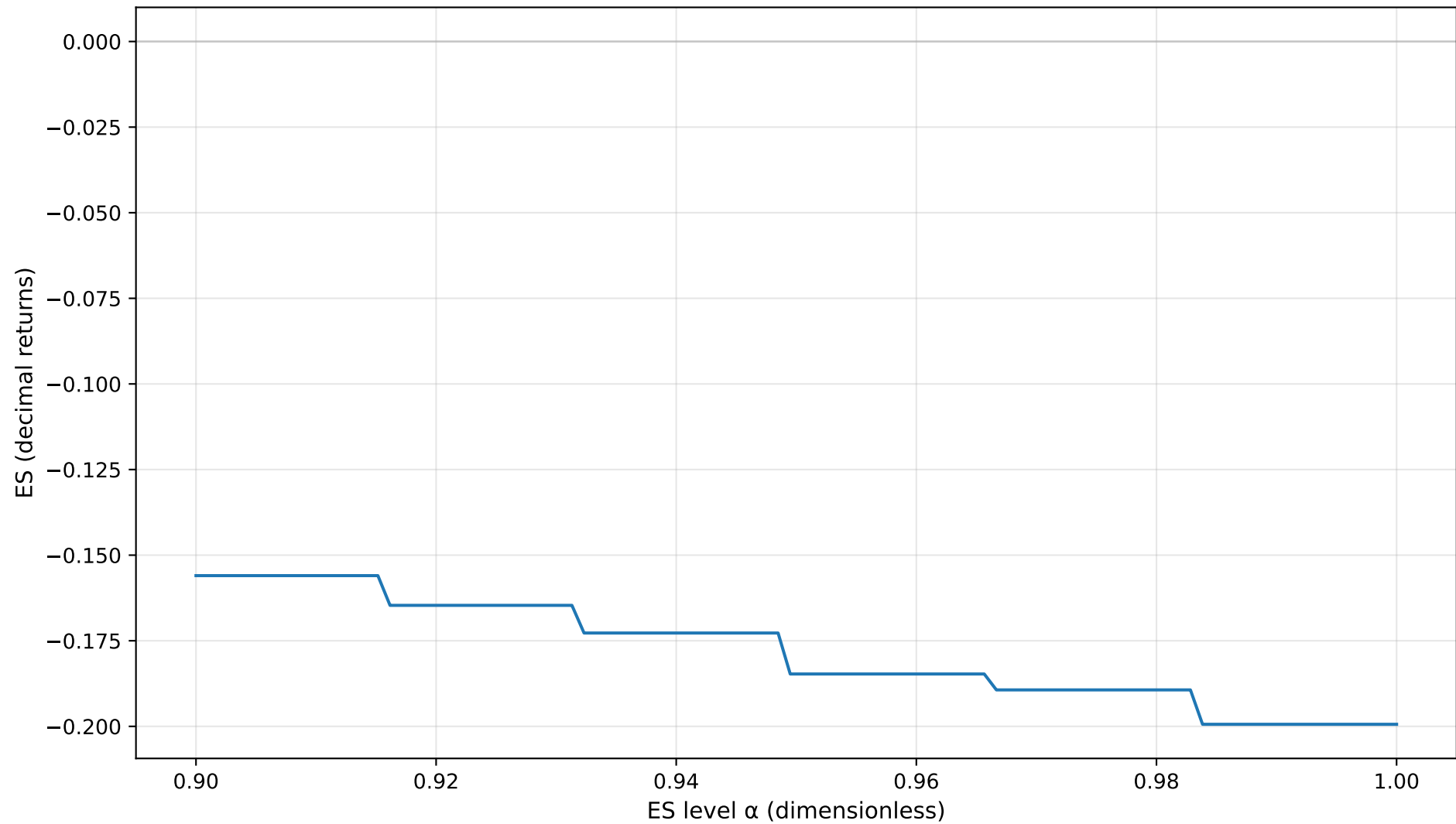
ES Curve (90-100%) — SUSPECT SCALE
