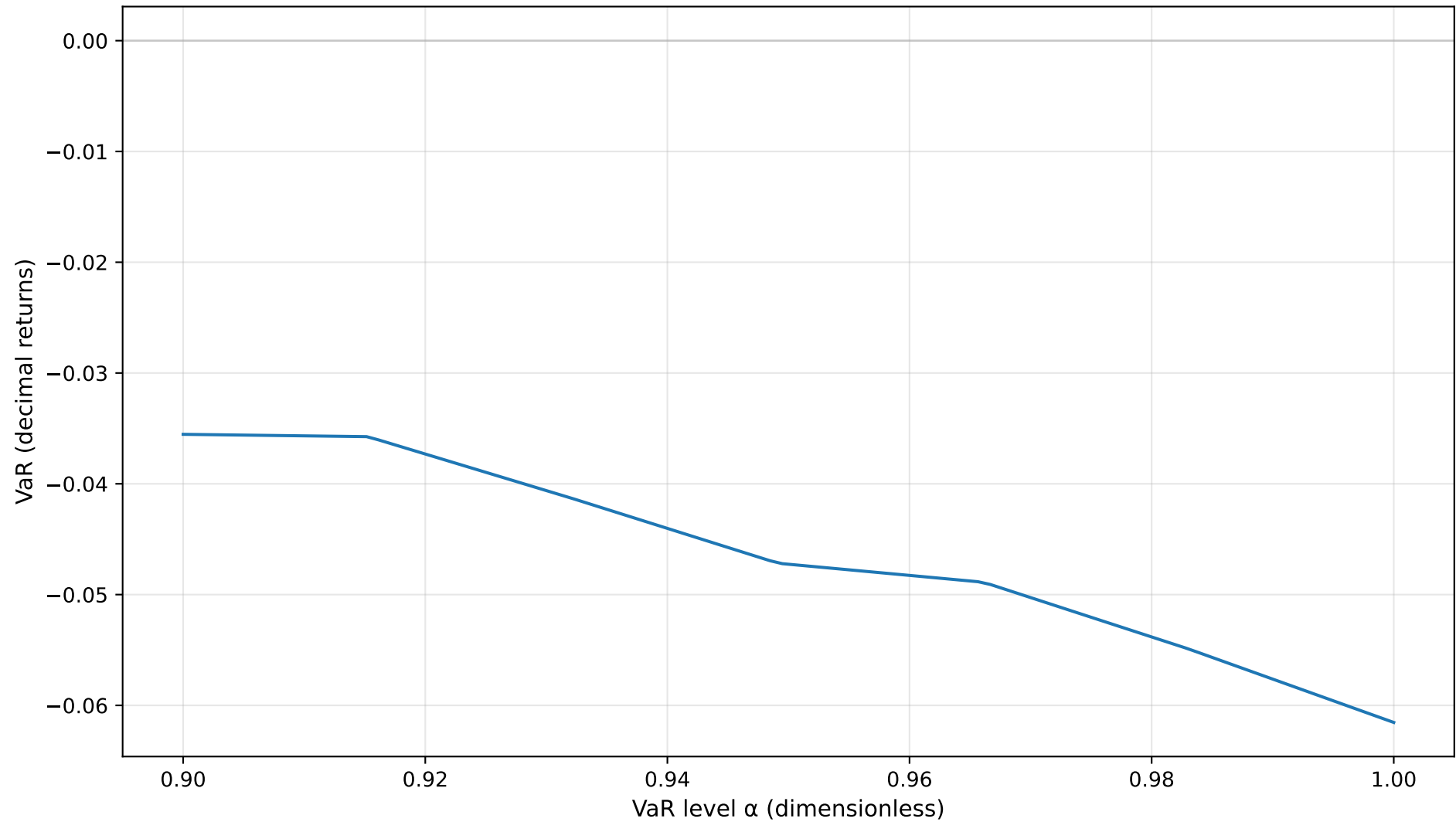
VaR Curve (90-100%)
