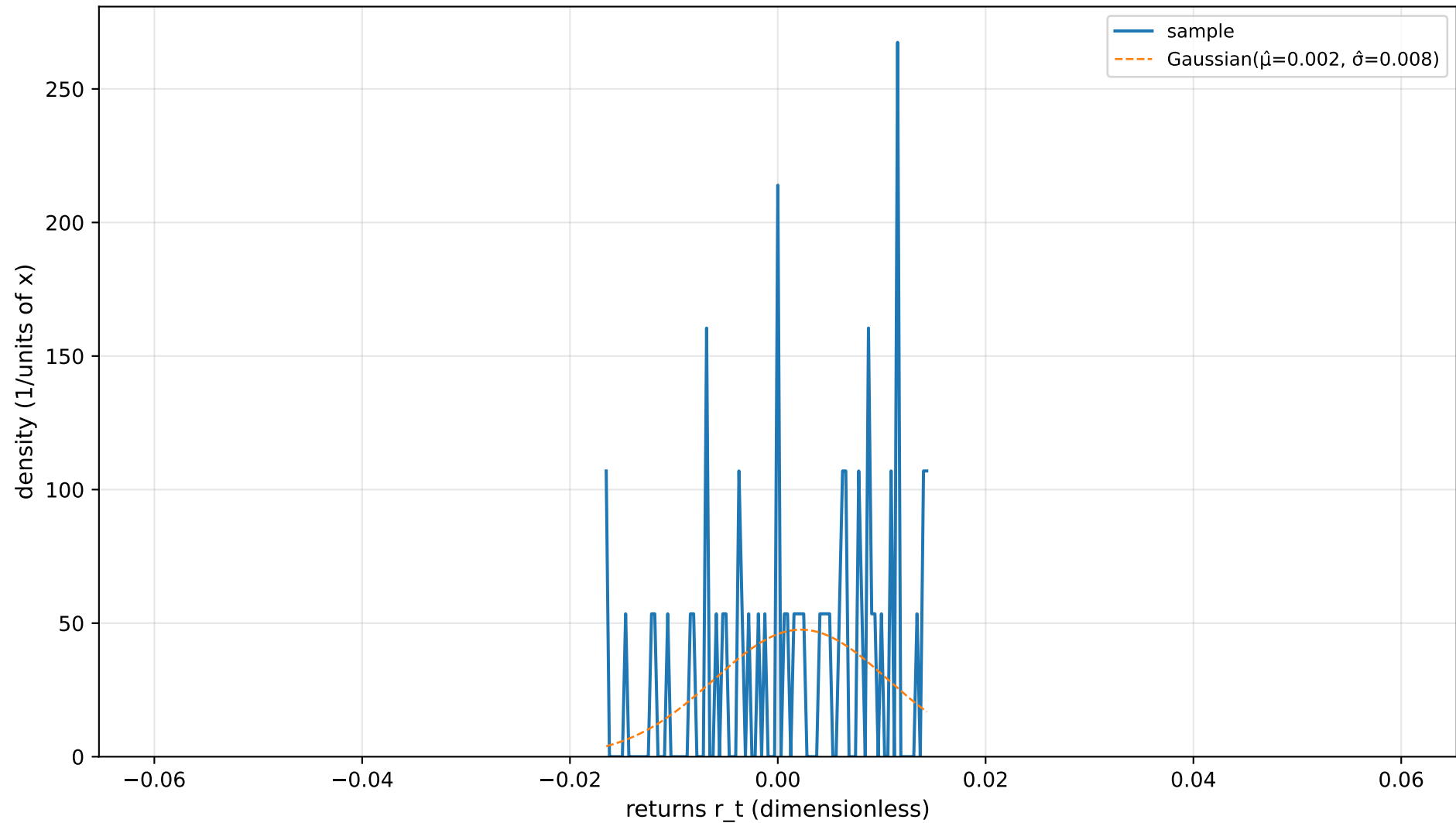
Density Overlay
