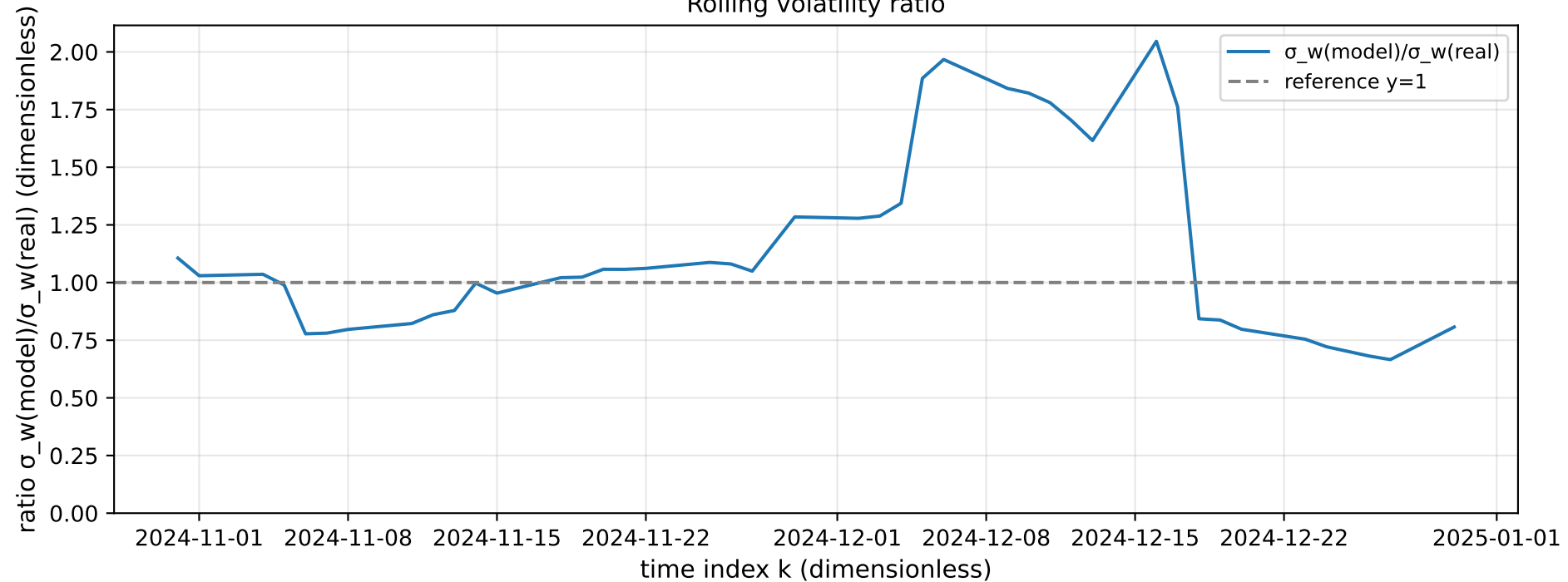
Rolling volatility ratio
