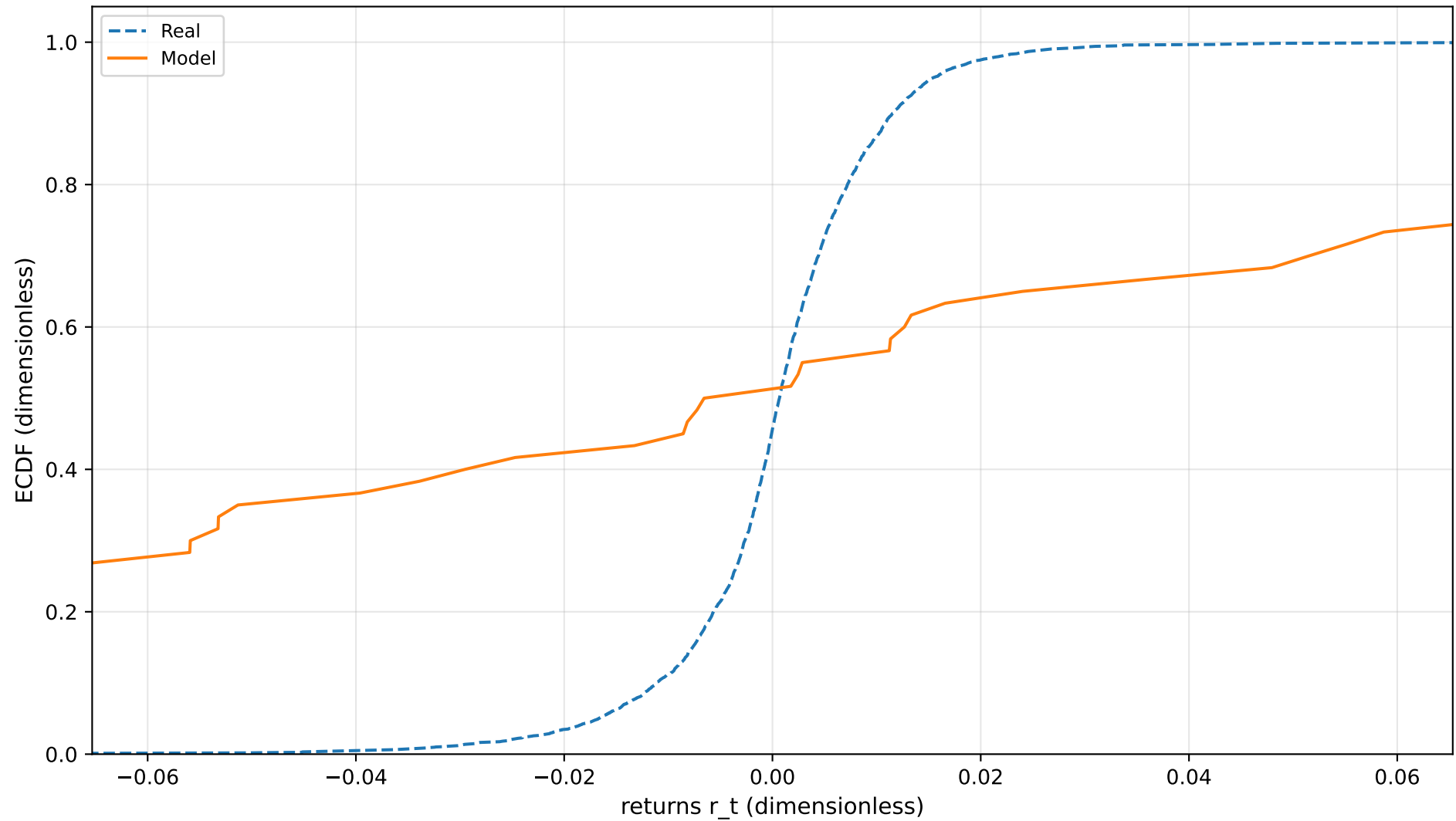
ECDF Overlay — SUSPECT SCALE
