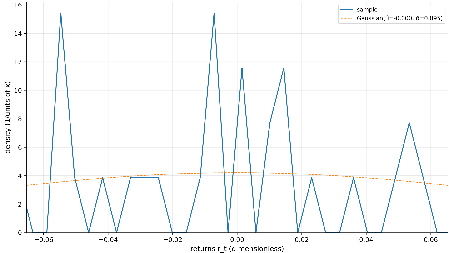
Density Overlay — SUSPECT SCALE
