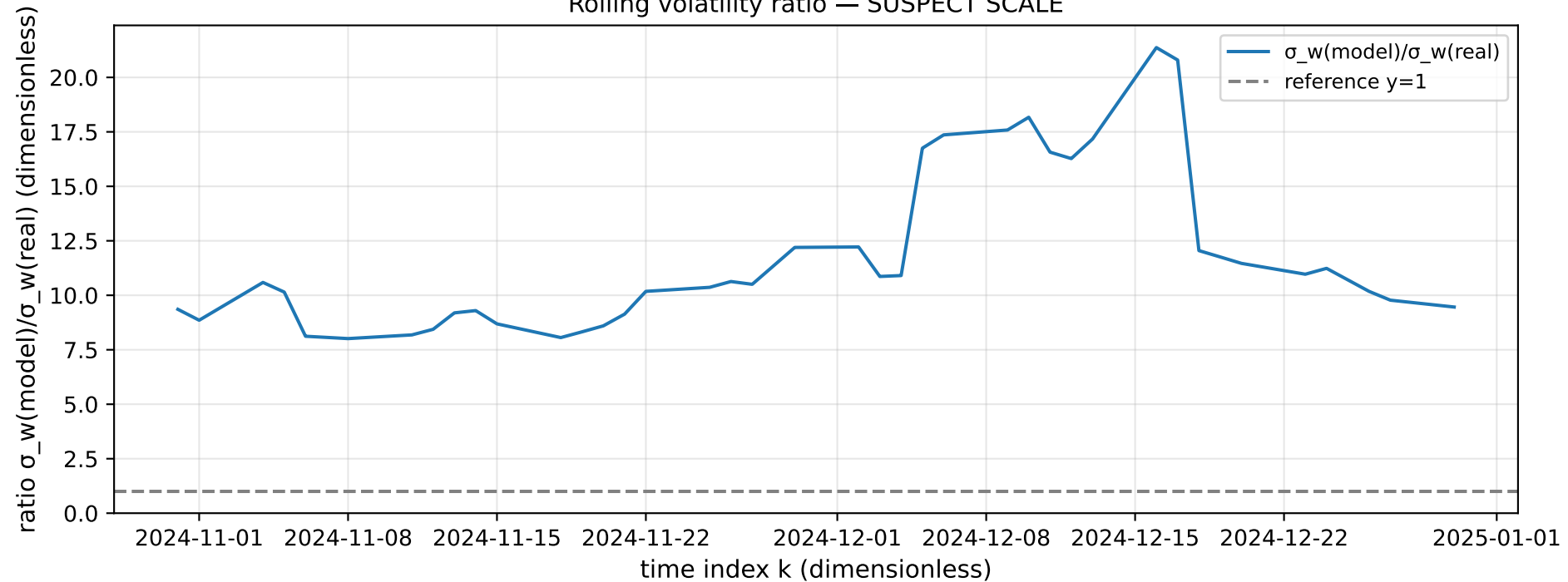
Rolling volatility ratio — SUSPECT SCALE
