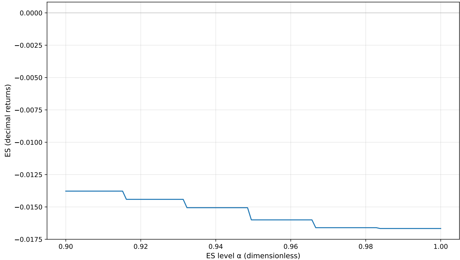
ES Curve (90-100%)
