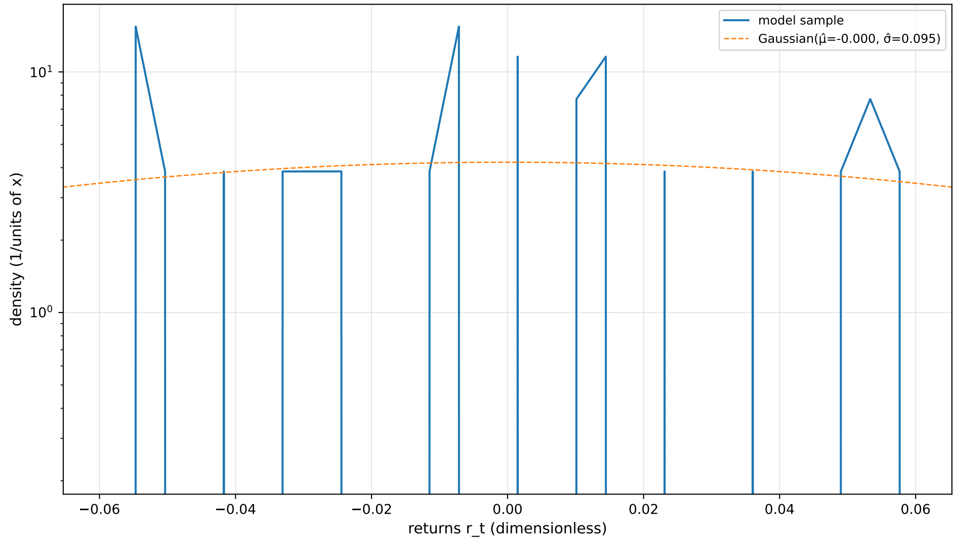
Histogram (log y-axis) — SUSPECT SCALE
