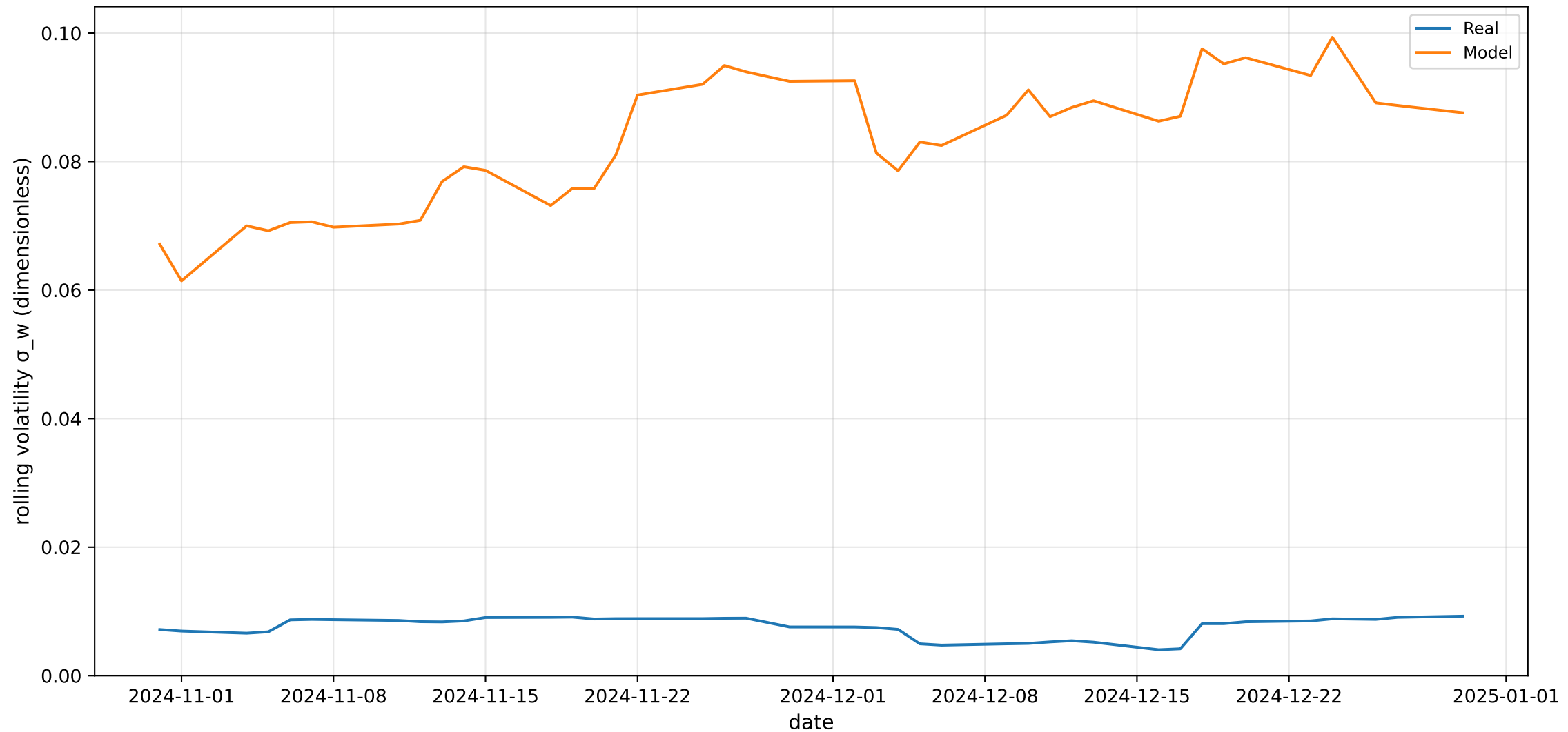
Rolling Volatility (window=20) — SUSPECT SCALE
