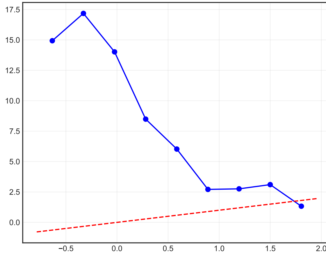
LLM Reliability
