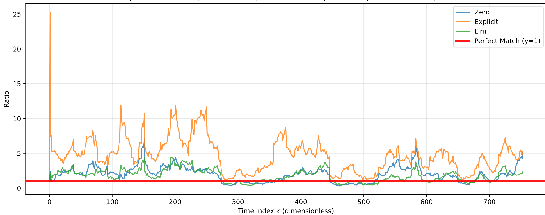
Volatility Ratios ( \sigma_w(\text{model})/\sigma_w(\text{real}) ) zero: \mu=1.98 , med=2.01, \rho=-0.11 ; explicit: \mu=4.67 , med=4.59, \rho=0.04 ; llm: \mu=1.78 , med=1.72, \rho=-0.03
