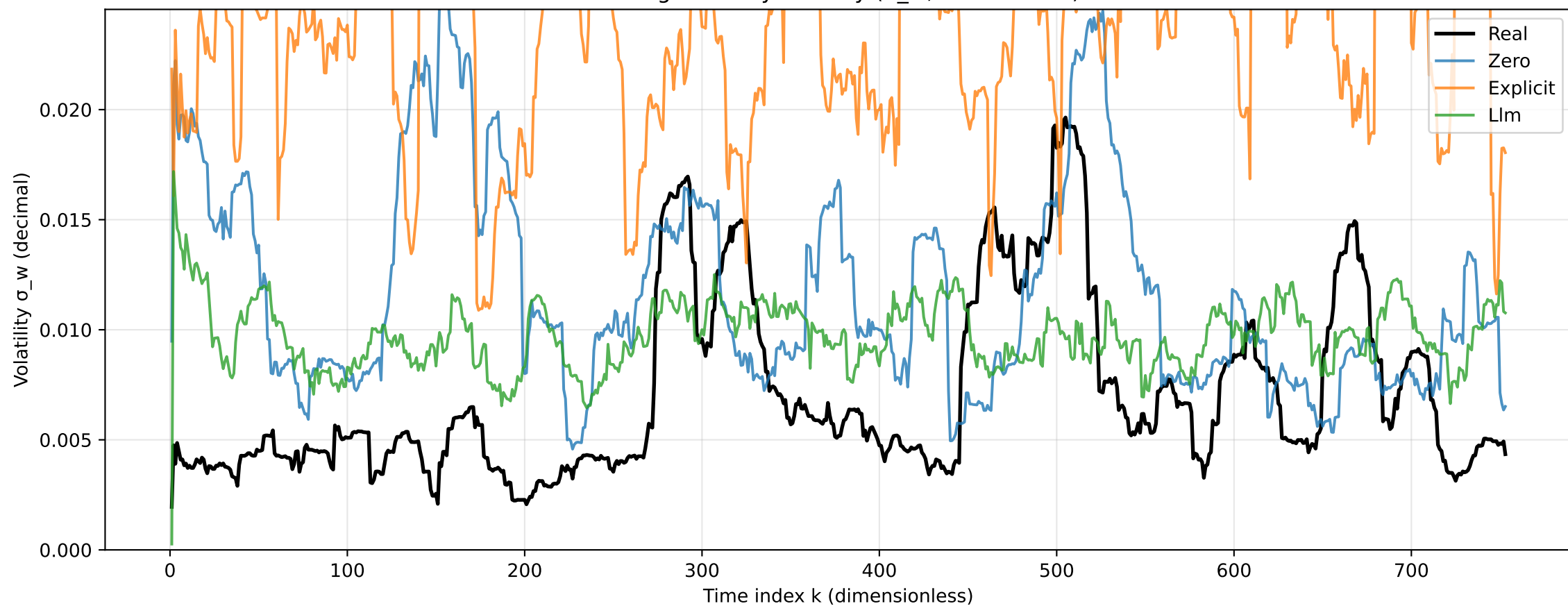
Volatility Ratios ( \sigma_w(\text{model})/\sigma_w(\text{real}) ) zero: \mu=2.17 , med=1.79, \rho=0.05 ; explicit: \mu=4.70 , med=4.34, \rho=-0.19 ; llm: \mu=1.76 , med=1.72, \rho=0.10
