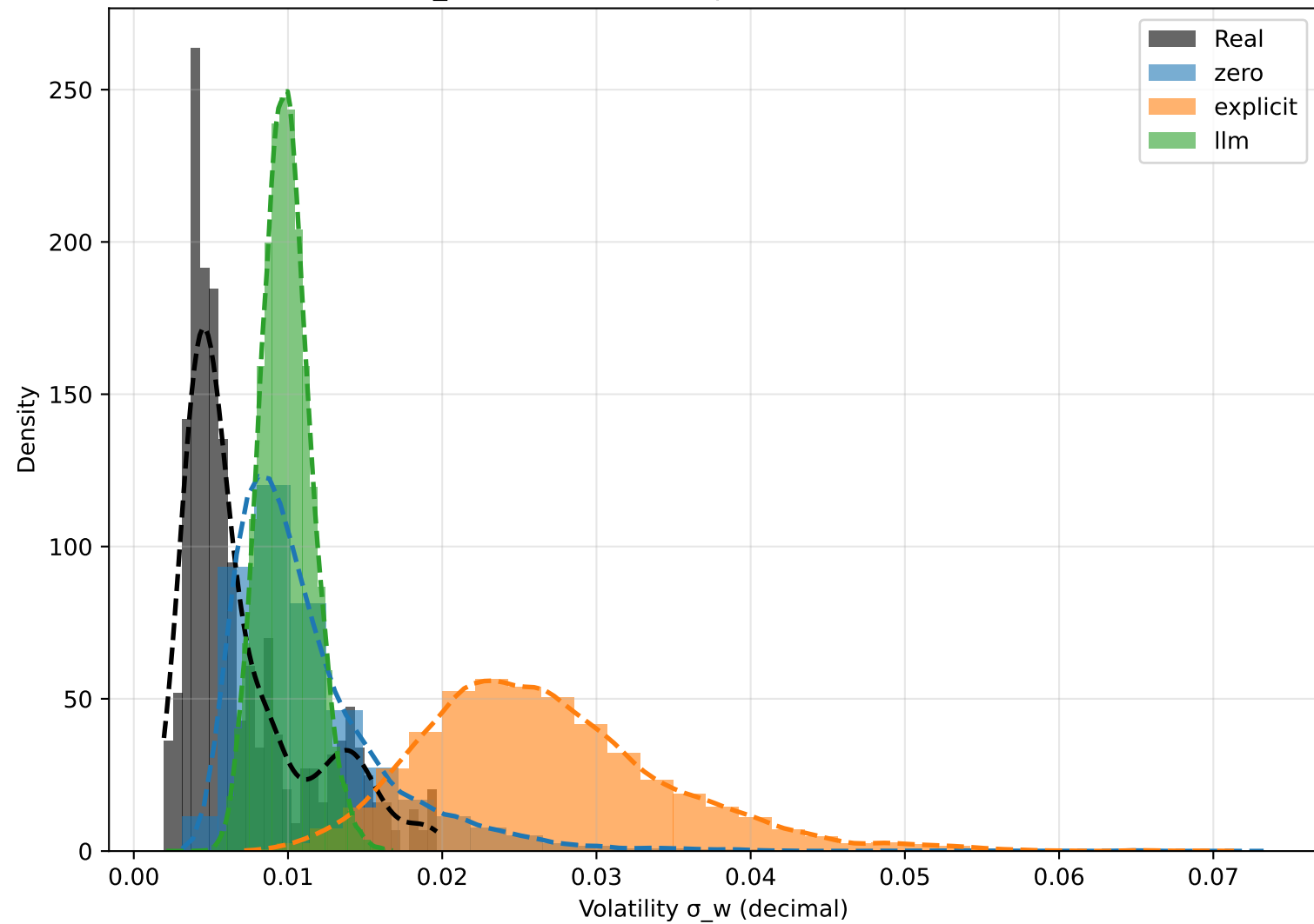
\sigma_w Distribution Comparison (window=20)
