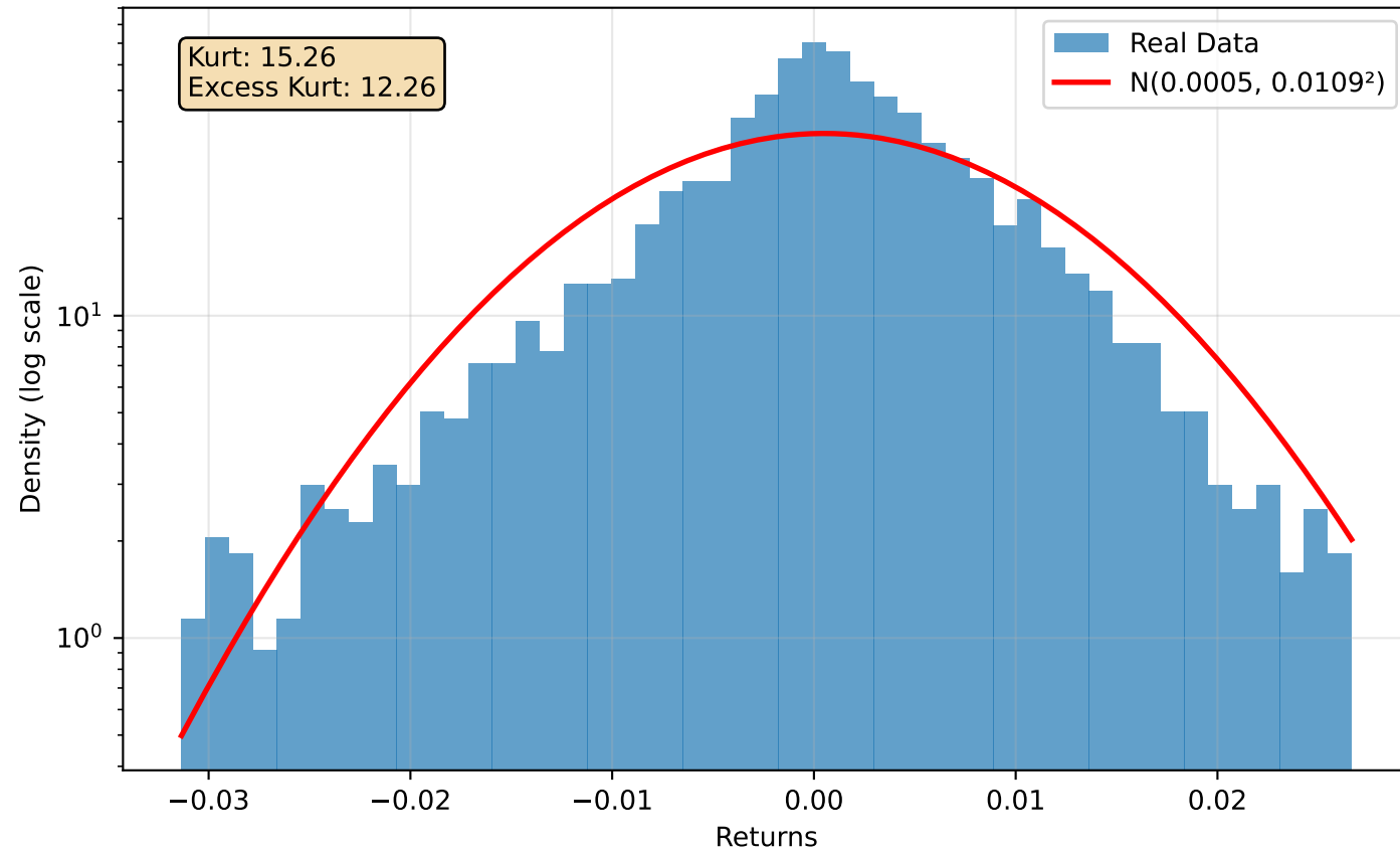
explicit Returns Distribution
