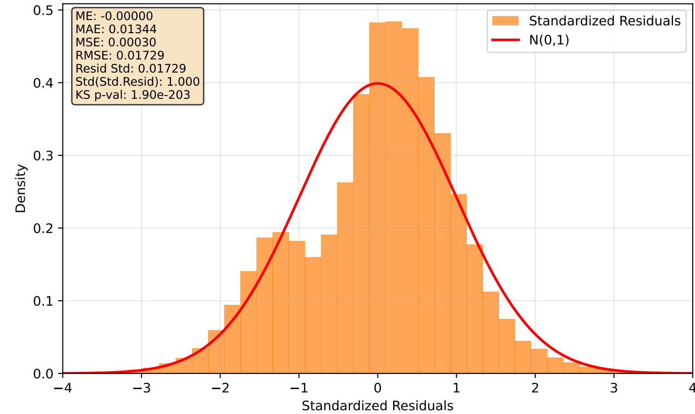
Ilm Standardized Residuals
