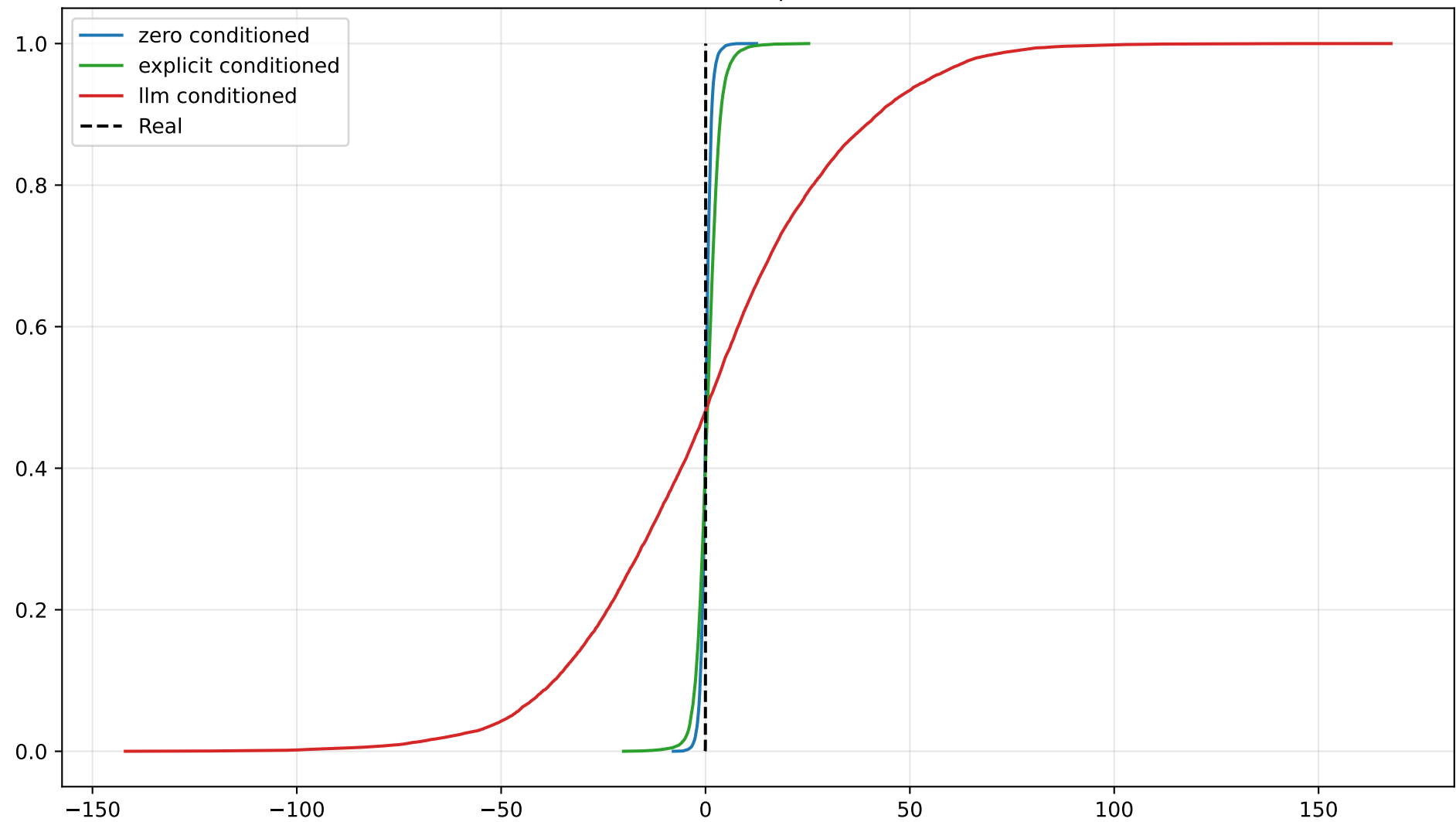
ECDF Comparison
