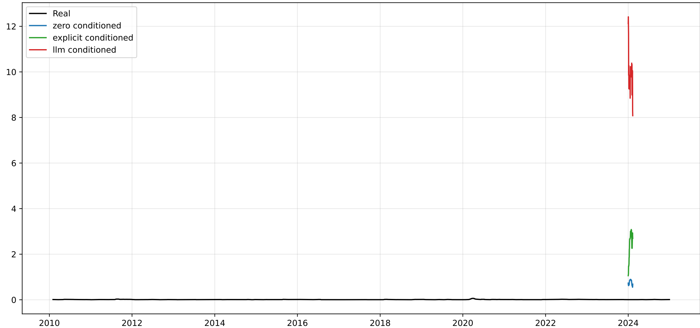
Rolling Volatility Comparison
