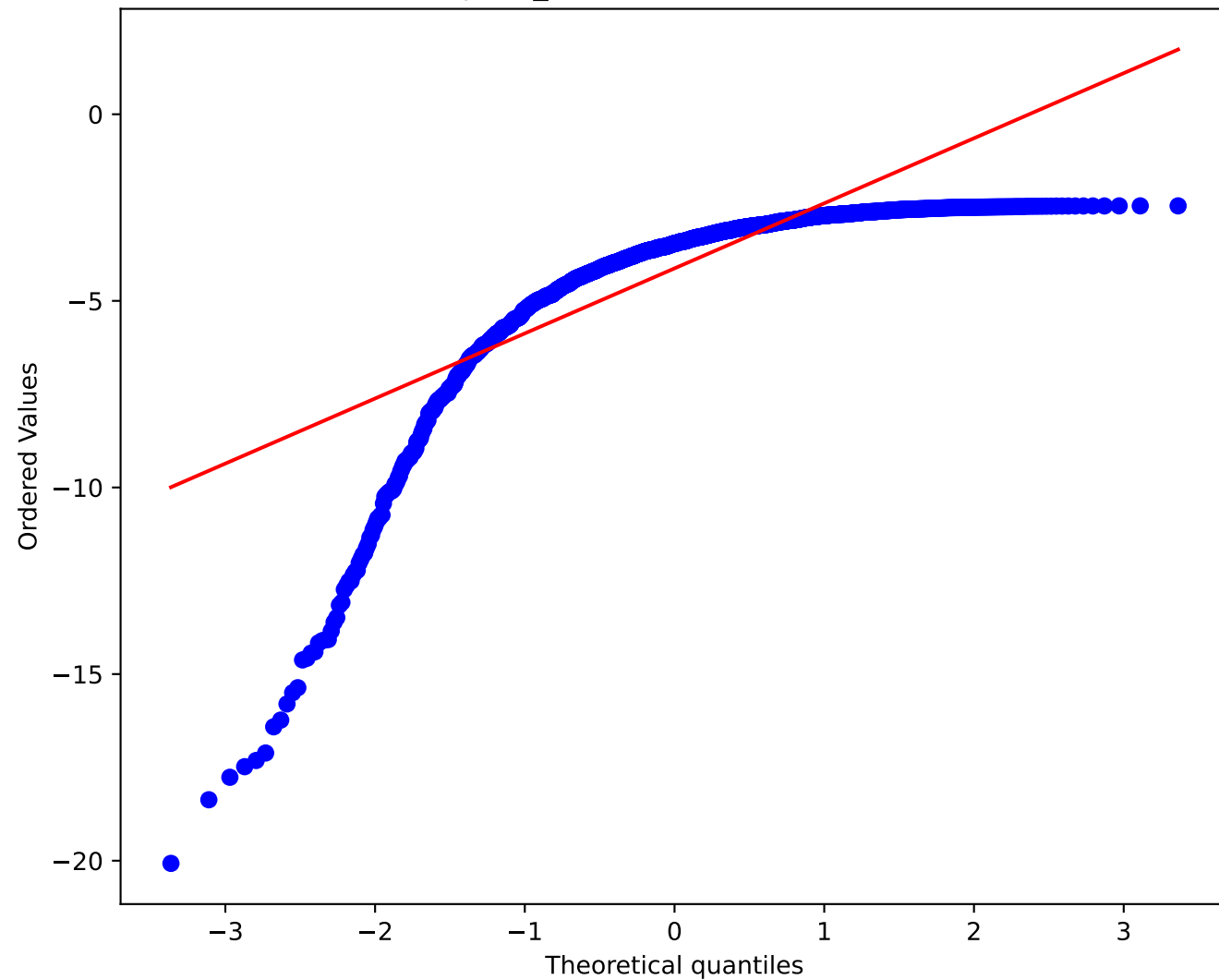
explicit_conditioned: Q-Q Left Tail
