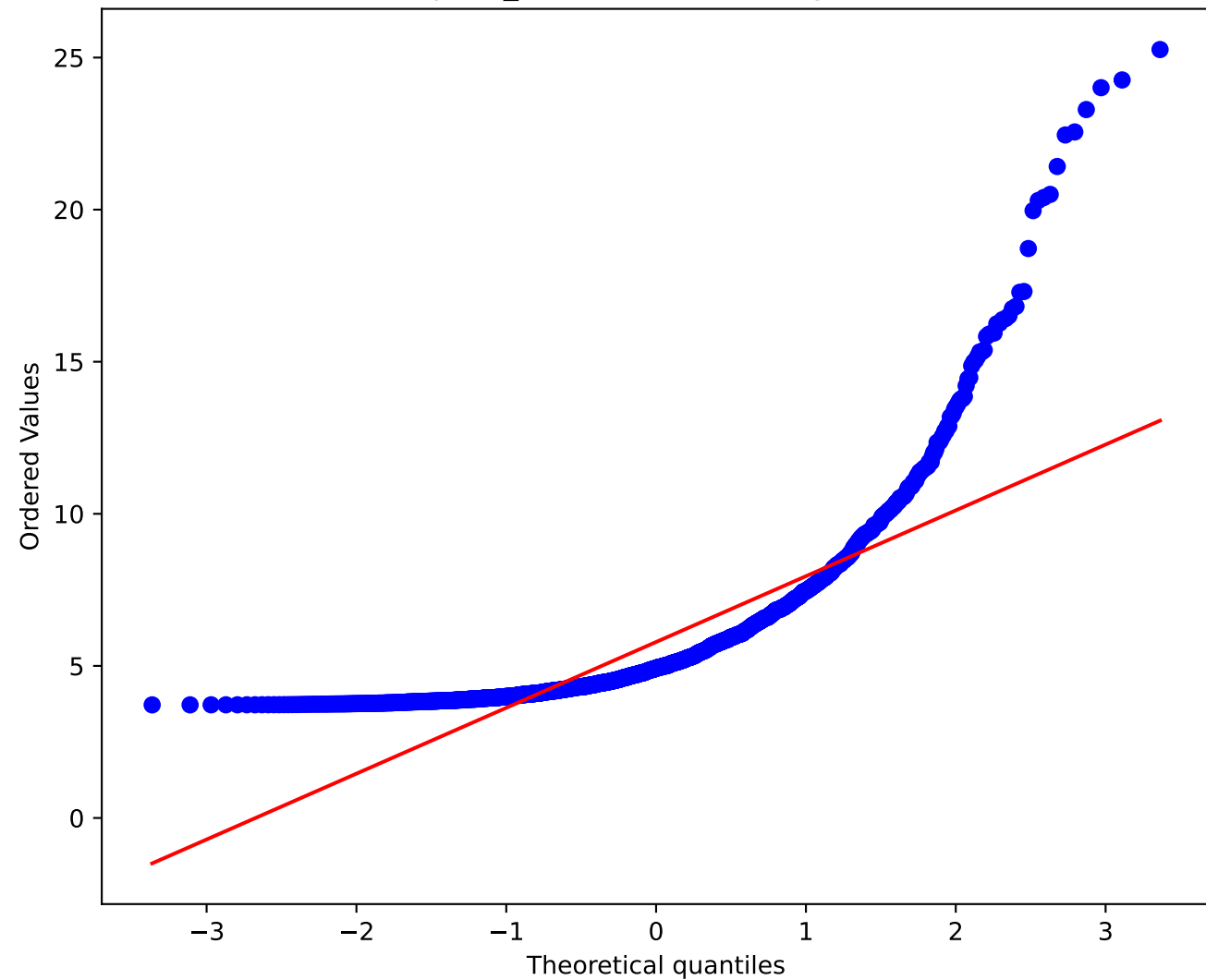
explicit_conditioned: Q-Q Right Tail
