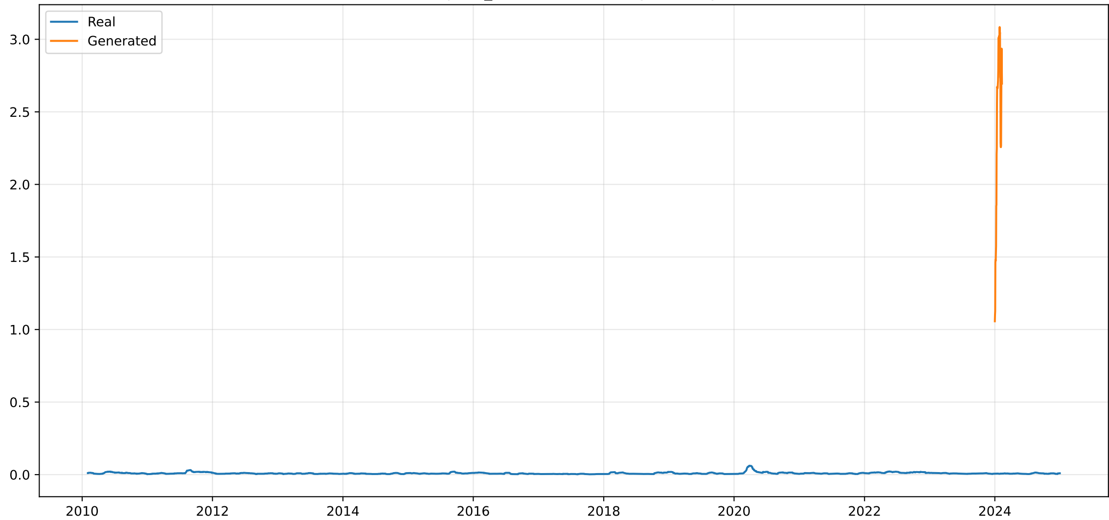
explicit_conditioned: Rolling Volatility
