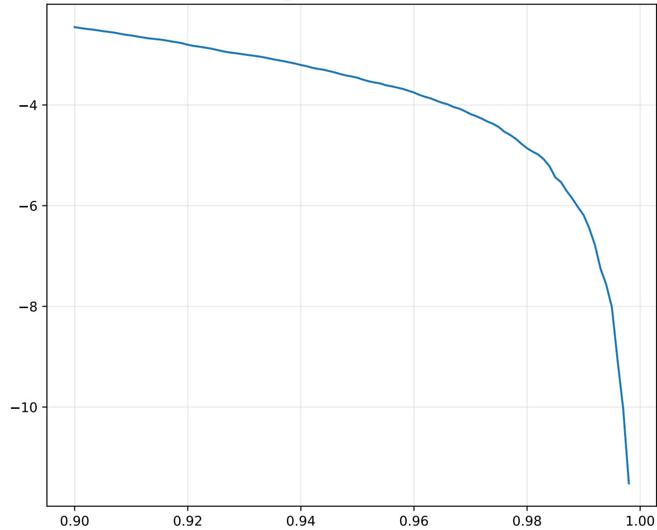
explicit_conditioned: VaR Curve
