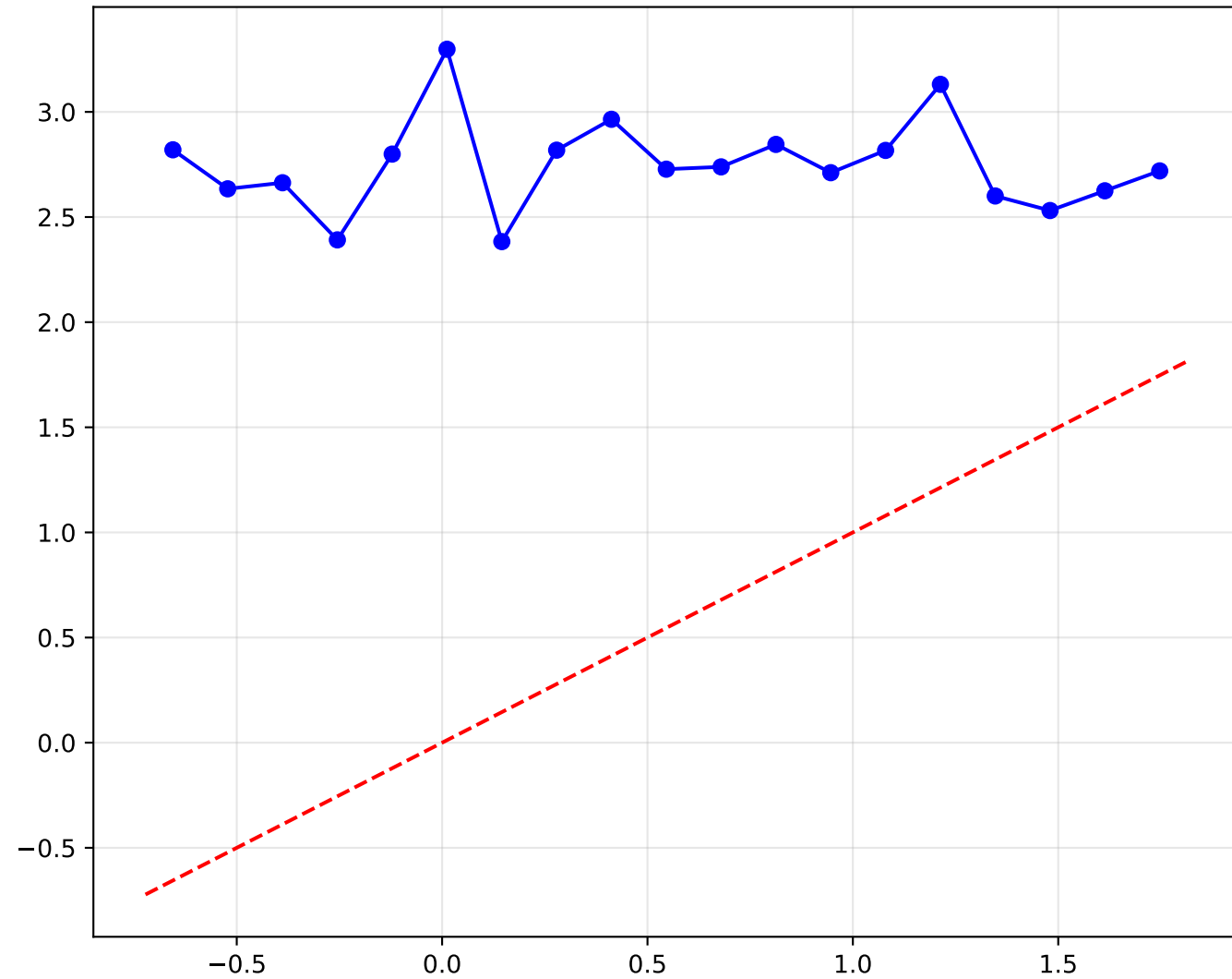
Reliability Curve
