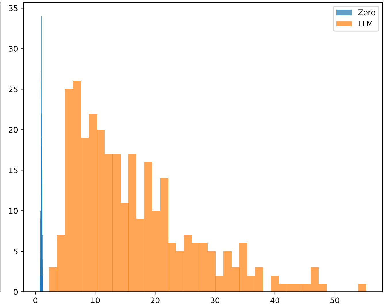
Ablation: Zero vs LLM
