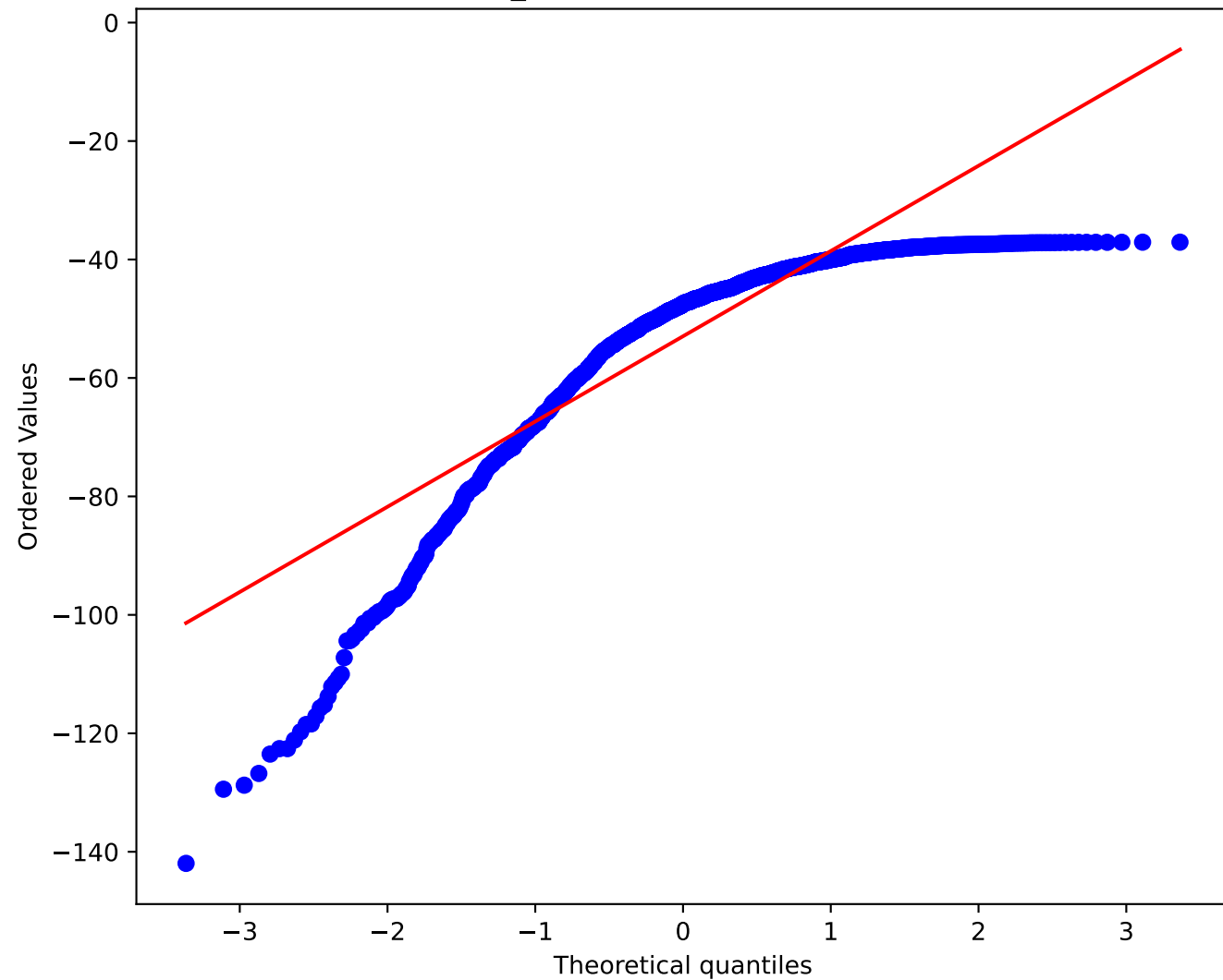
llm_conditioned: Q-Q Left Tail
