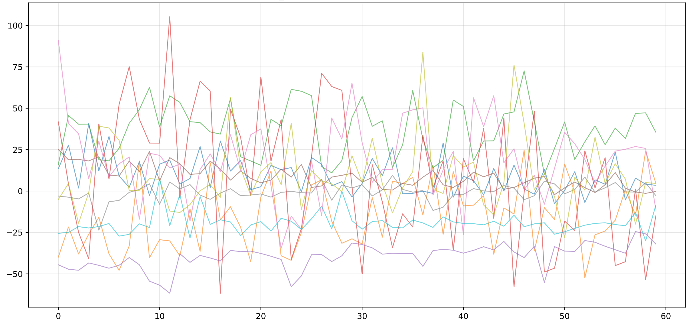
l1m_conditioned: Sample Paths (n=10)
