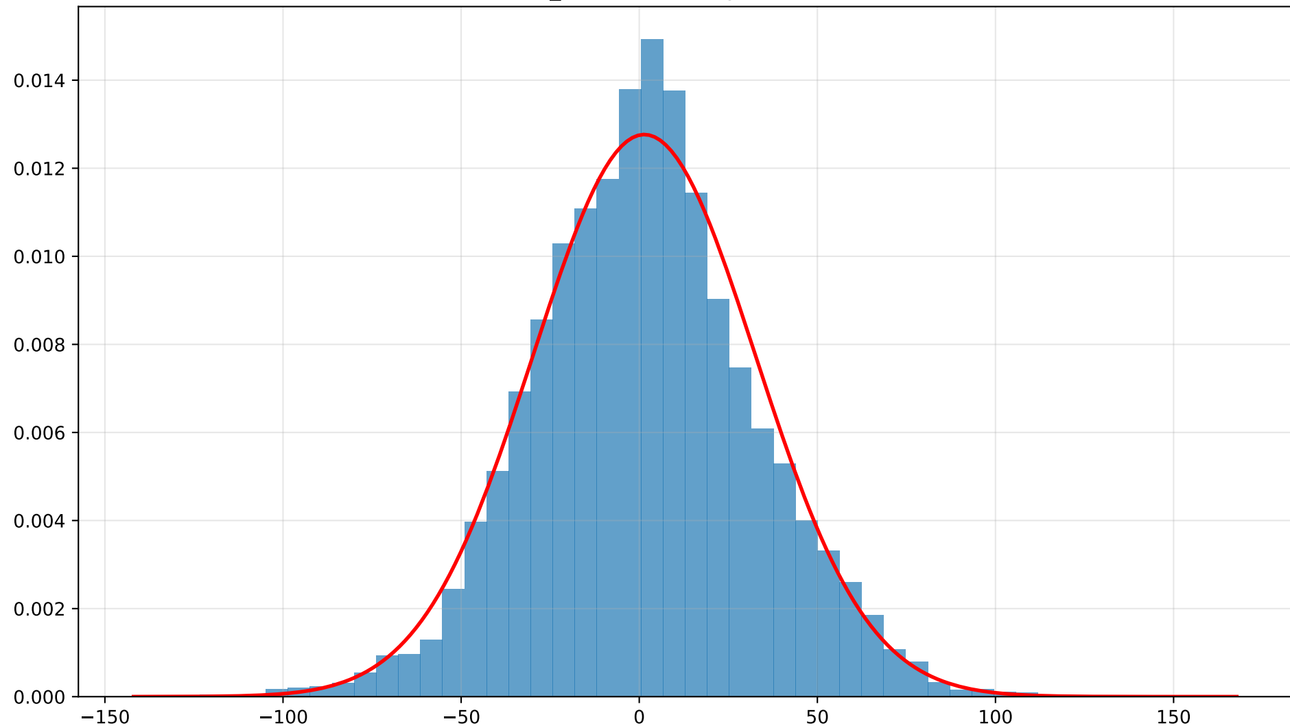
l1m_conditioned: Stylised Facts
