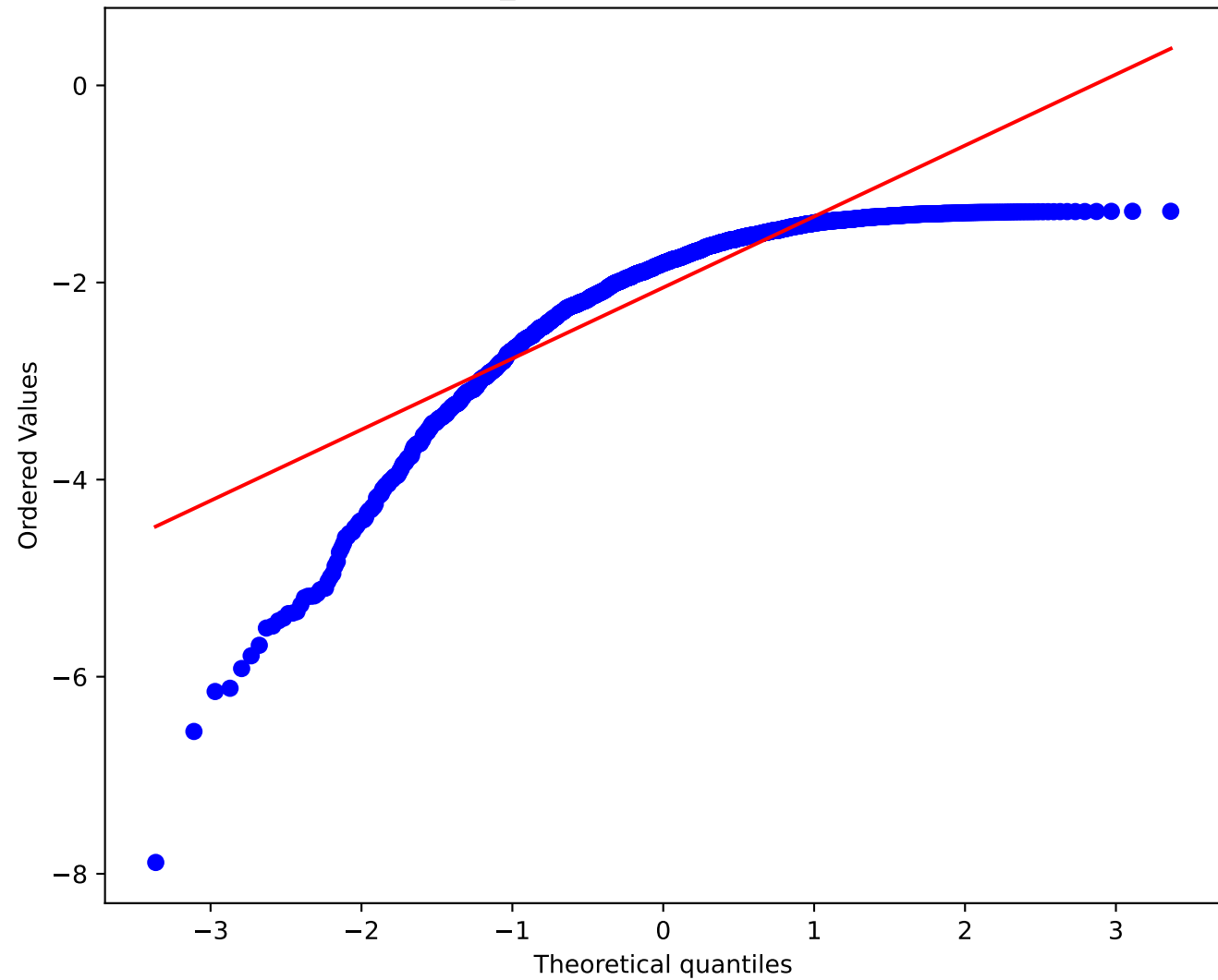
zero_conditioned: Q-Q Left Tail
