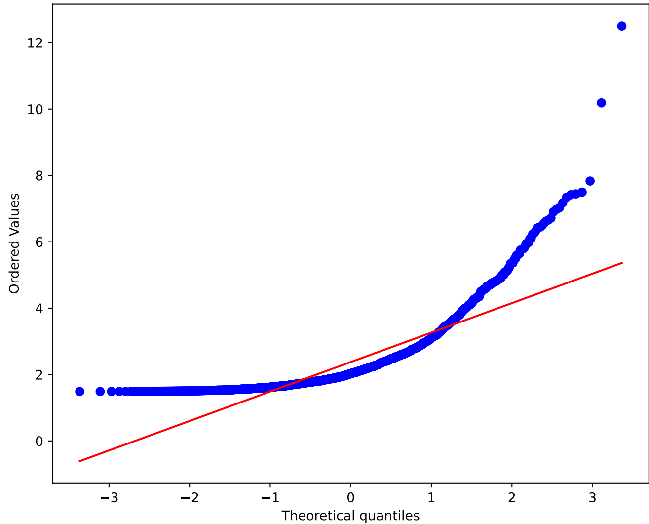
zero_conditioned: Q-Q Right Tail
