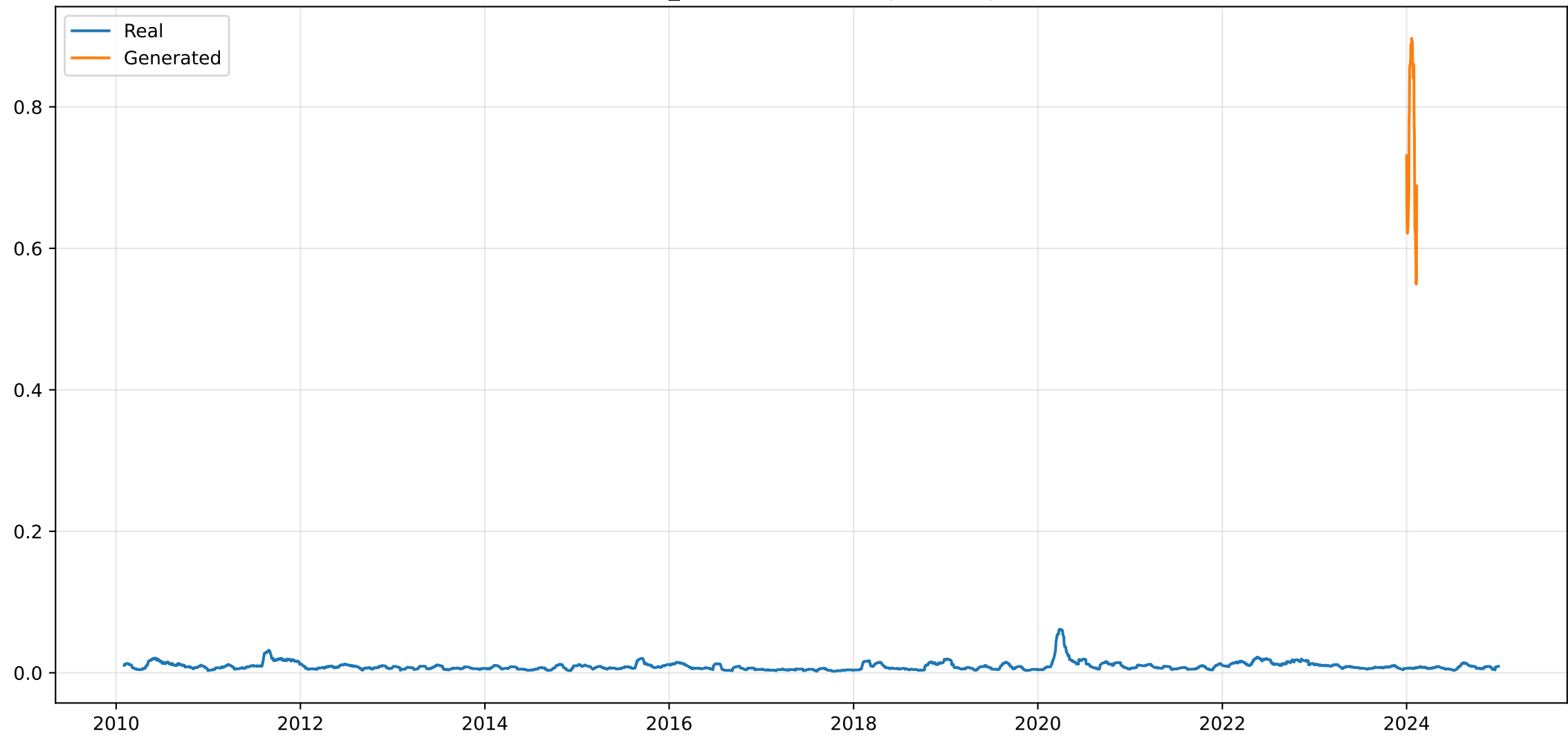
zero_conditioned: Rolling Volatility
