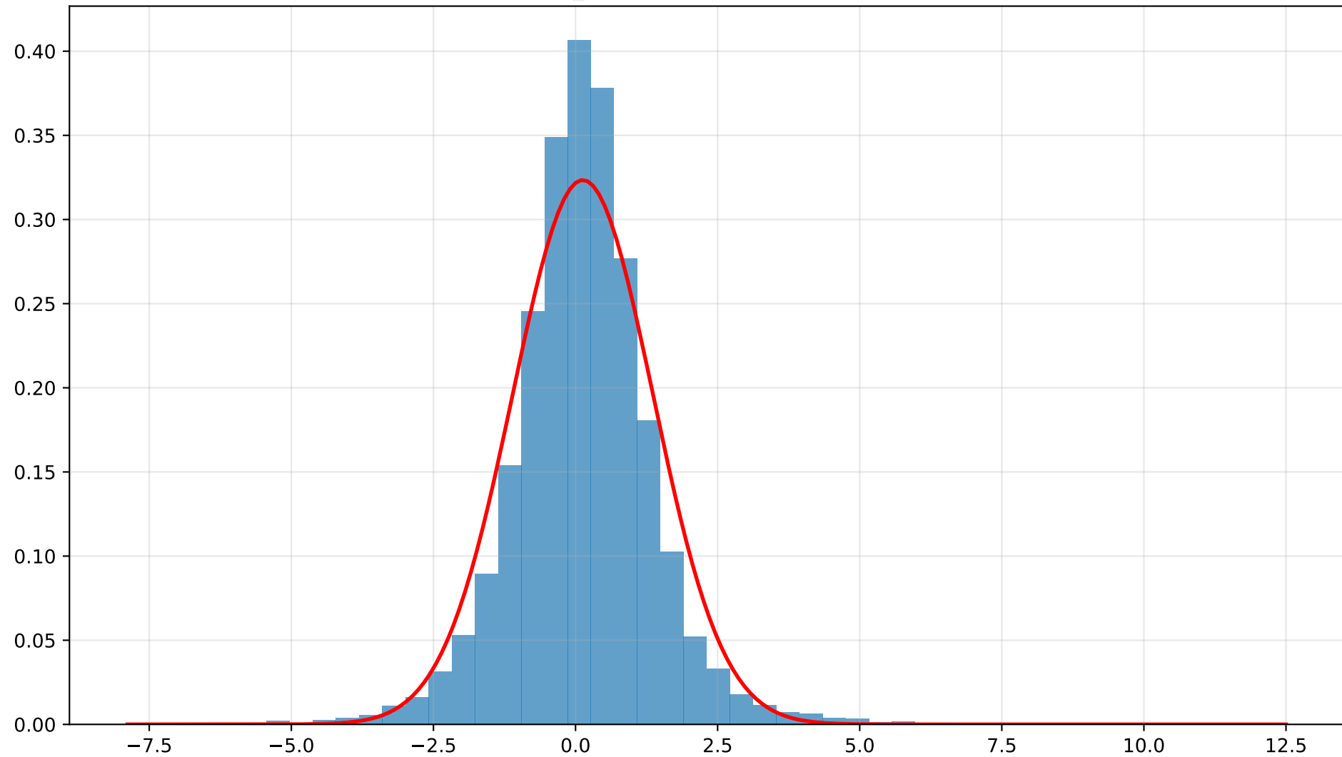
zero_conditioned: Stylised Facts
