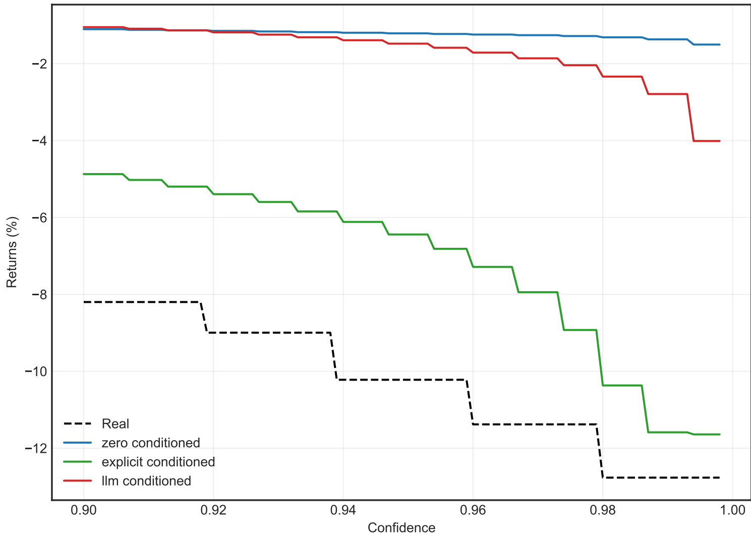
Crisis ES Curve
