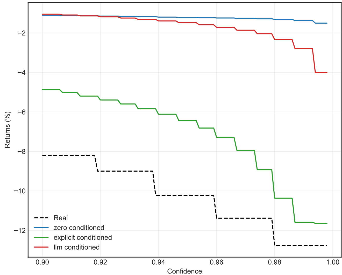
Crisis ES Curve
