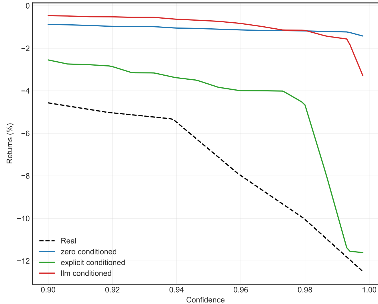
Crisis VaR Curve
