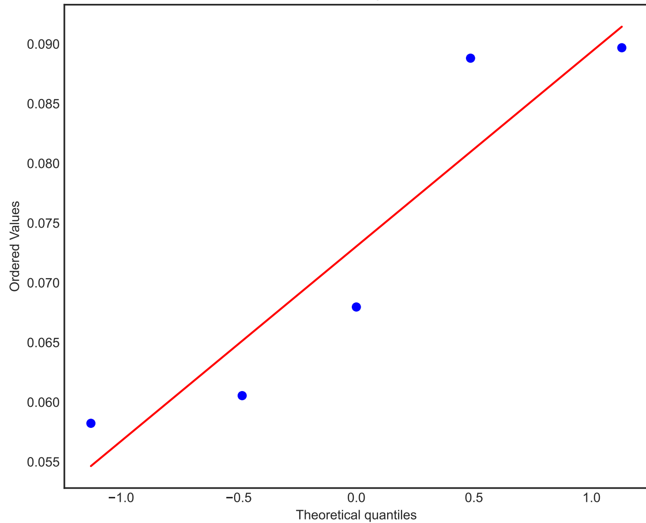
real: Q-Q Right Tail
