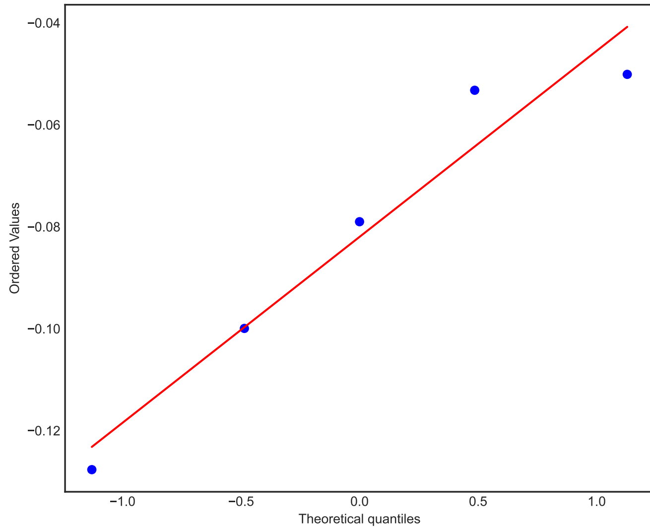
real: Q-Q Left Tail
