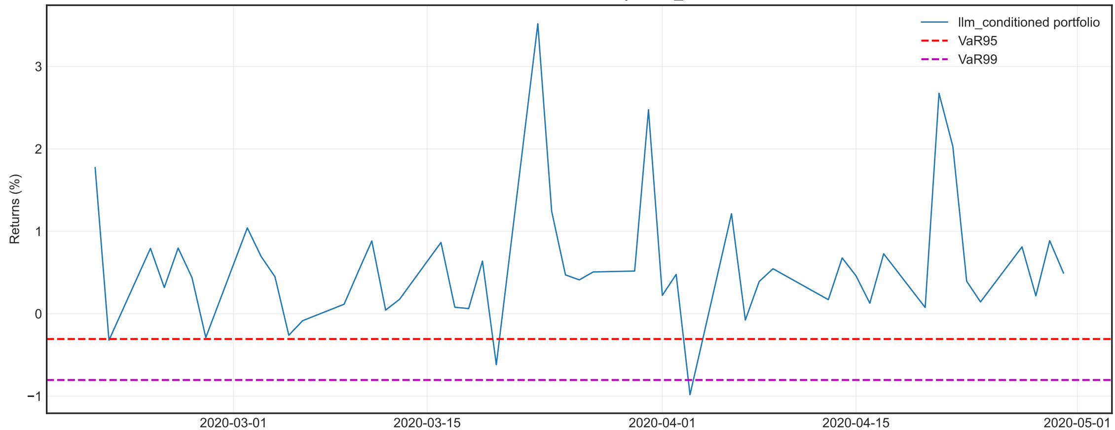
Portfolio Losses with VaR Overlays - l1m_conditioned
