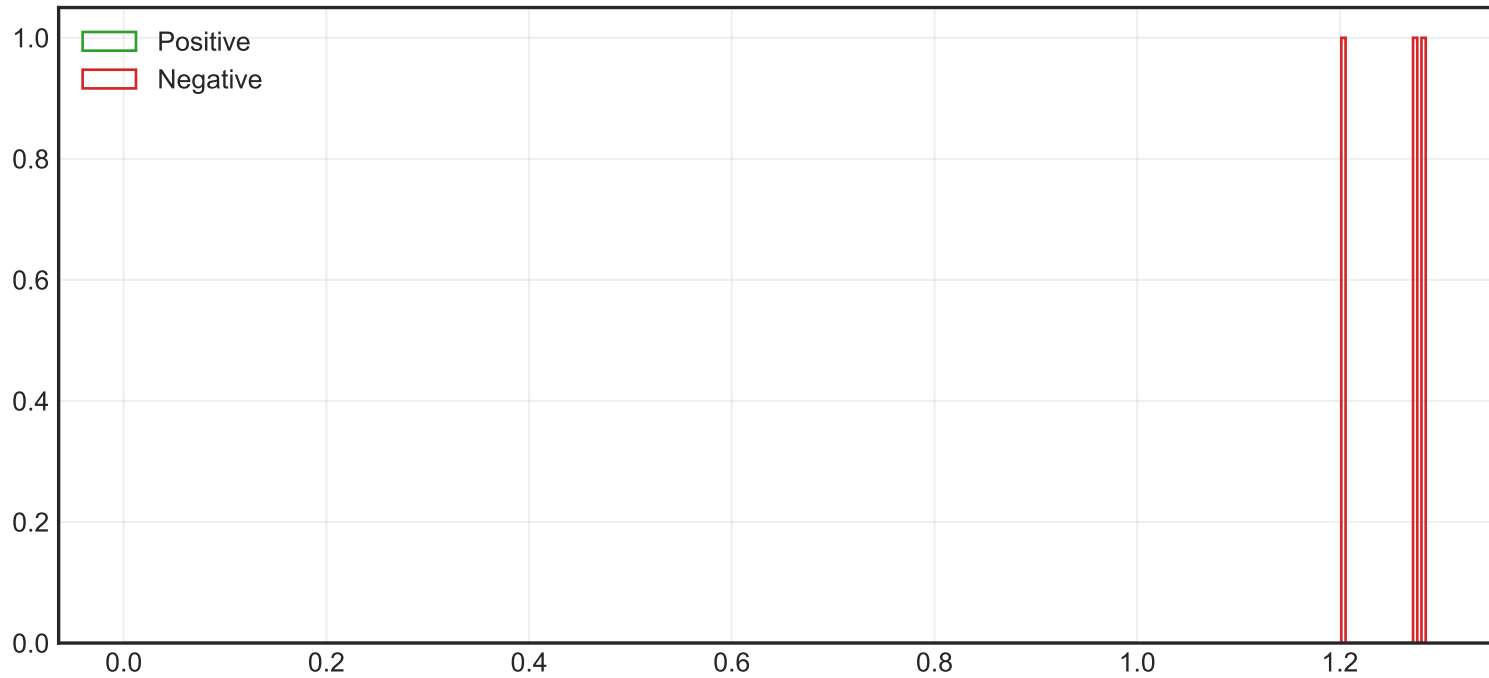
LLM Sentiment Buckets: Realized Volatility
