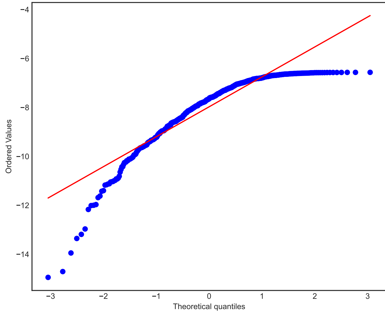
llm_conditioned: Q-Q Left Tail
