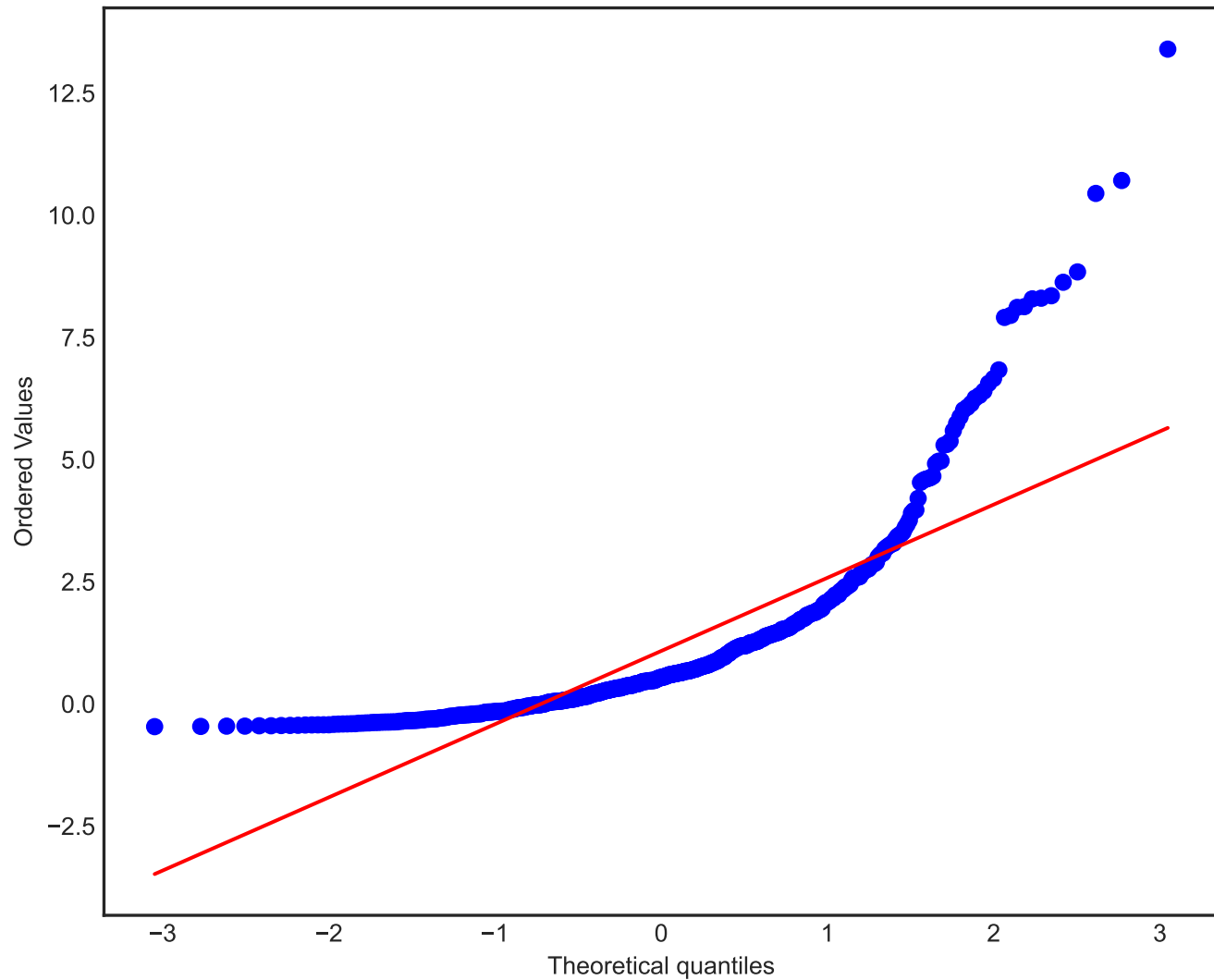
llm_conditioned: Q-Q Right Tail
