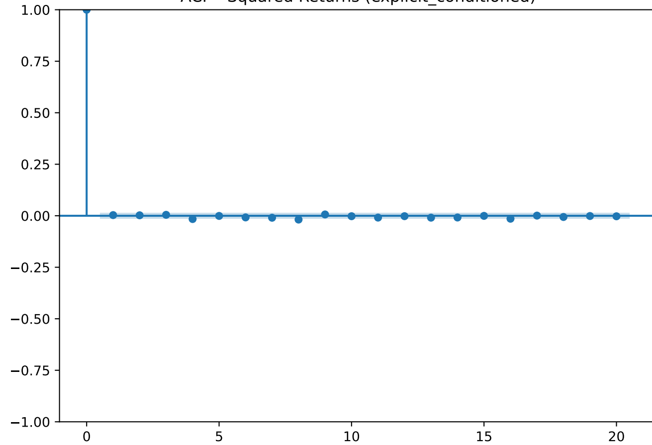
ACF - Squared Returns (explicit_conditioned)
