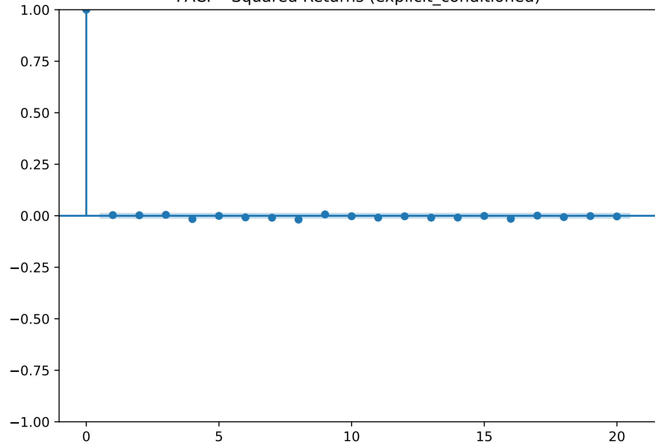
PACF - Squared Returns (explicit_conditioned)
