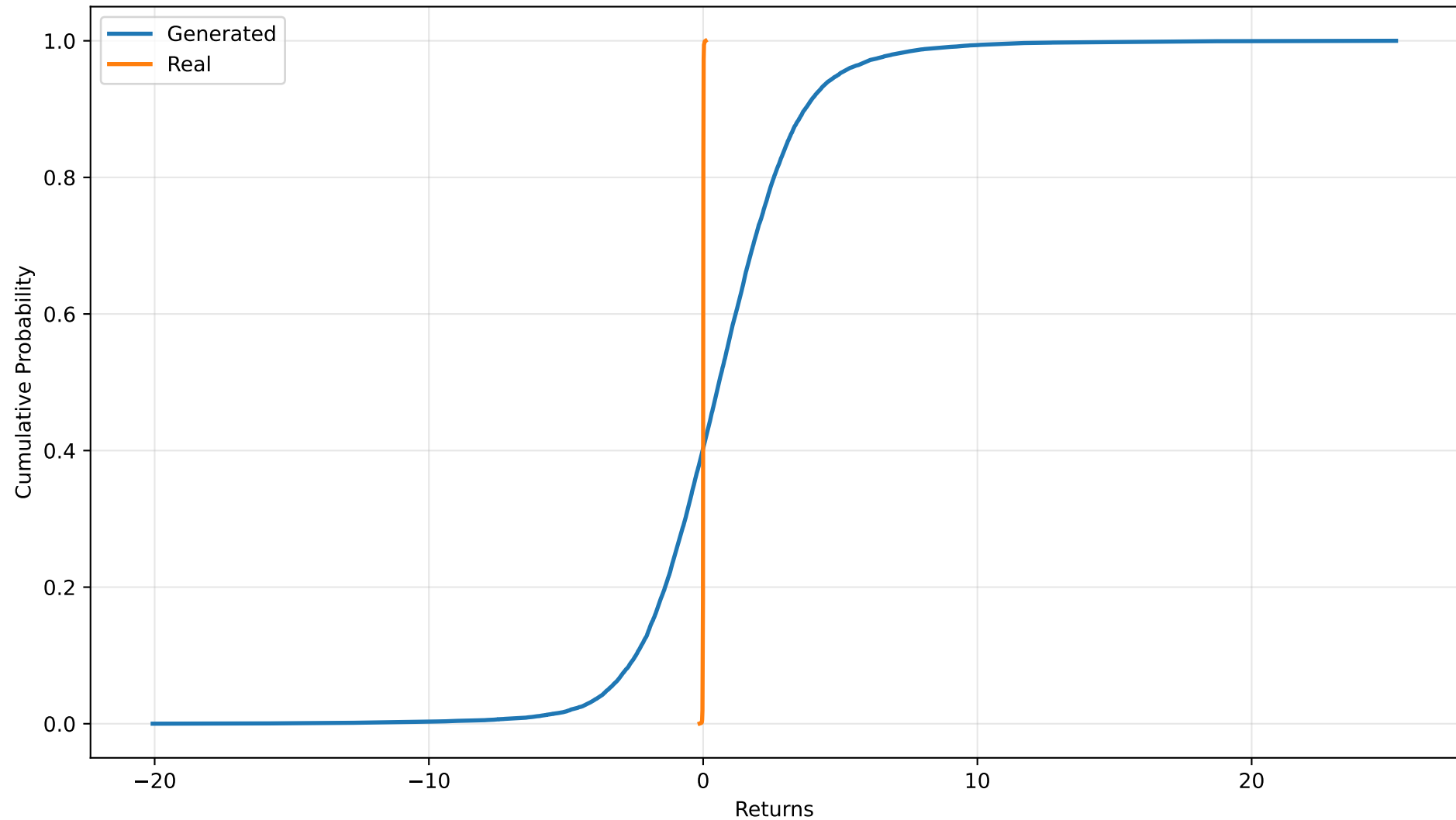
Explicit Conditioned: ECDF Comparison
