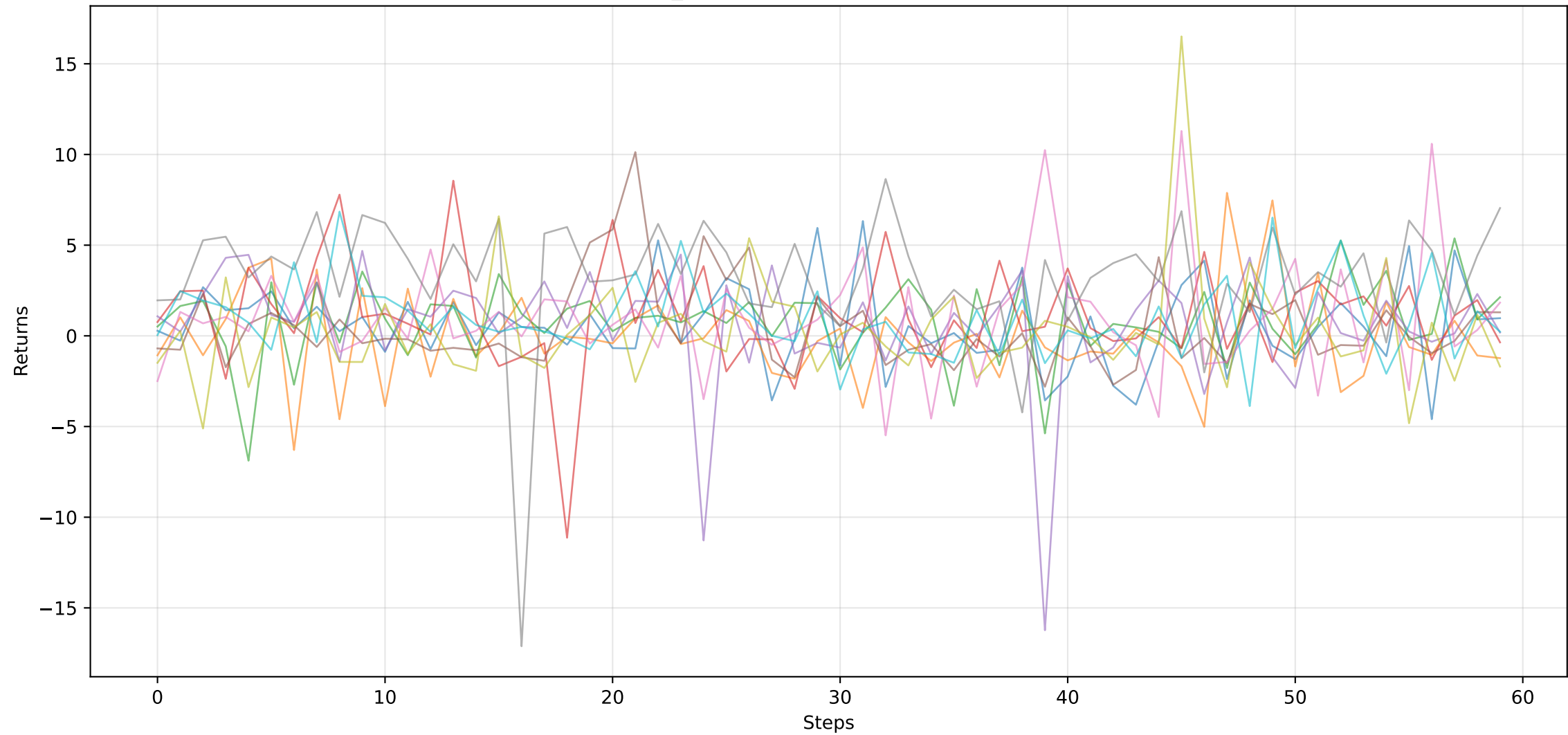
Explicit_Conditioned: Sample Paths (n=10)
